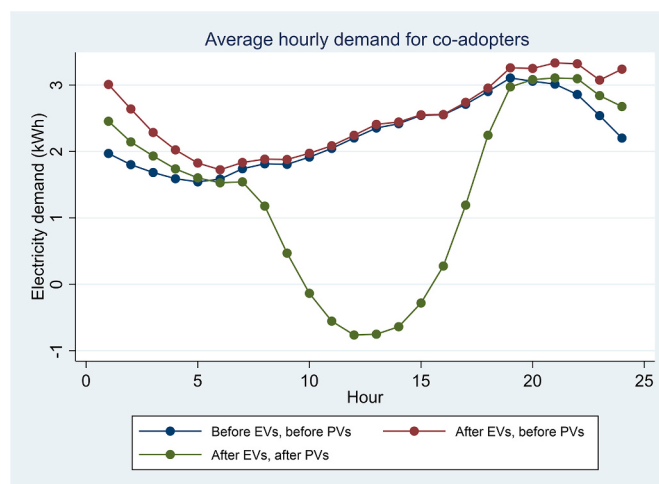
Fig. A2. Net delivered hourly electricity demand after EV/PV adoption for co-adopters.
