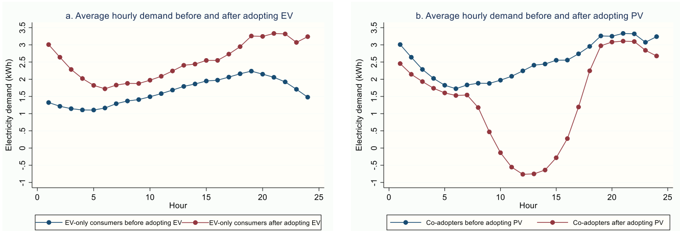
Fig. 3. Descriptive summary of net delivered hourly electricity demand after EV/PV adoption.
