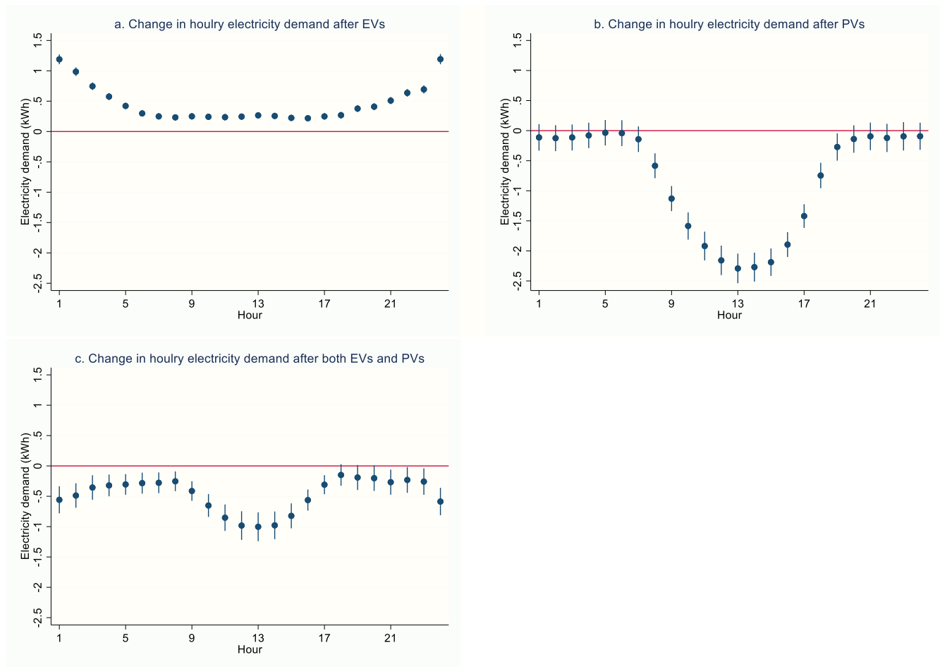
Fig. 7. Changes in hourly electricity demand after EV and PV adoption.
