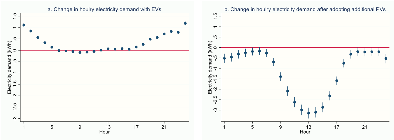
Fig. 5. Changes in hourly electricity demand after EV adoption and additional PV adoption.
