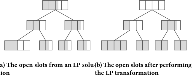
Figure 2: An example of a tree before and after running the LP transformation in Lemma 1. The dark slots represent slots have jobs scheduled in them, and the white slots are closed.
