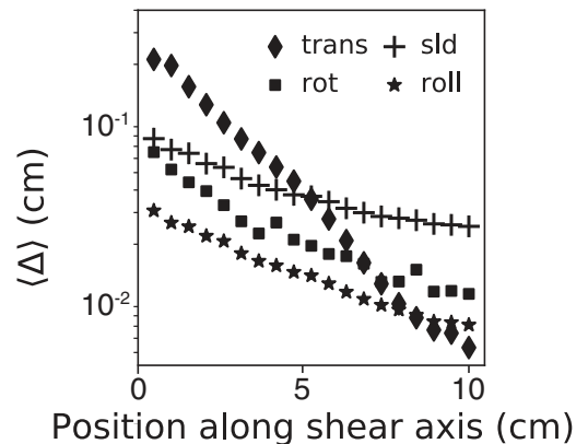
FIG. 4. Translations, rotations, sliding, and rolling as functions of position along the shear axis. Data are taken at full compression (from the middle of a cycle). The shear axis lies perpendicularly to the shear zone's striations (see Fig. 3). The sliding and rolling displacements result from summing the displacements across the first half of the time steps.
