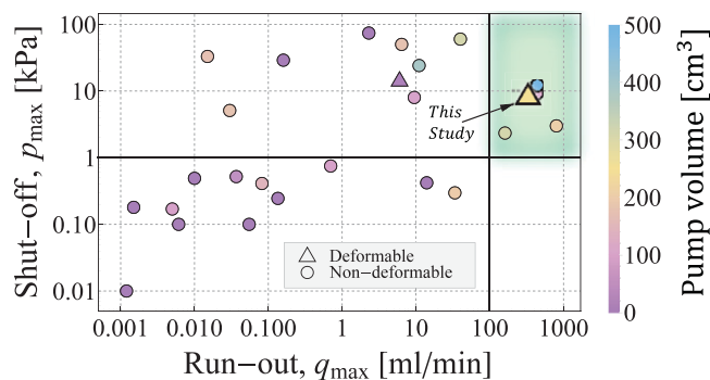
Fig. 1. Shut-off (max pressure, no flow) vs. run-out (max flow, no back-pressure) performance of comparable state-of-the-art systems. Visualization of novelty, largest work-point reported to date for pumps that operate under large deformations (of its own length scale). All other pump technologies in its performance order-of-magnitude are nondeformable pumps.
