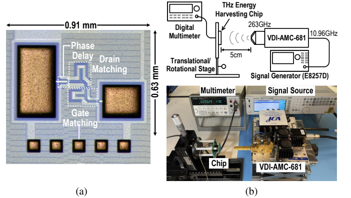
Fig. 7. (a) Chip micrograph. (b) Diagram and photo of the test setup.
