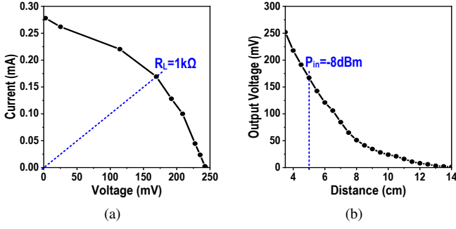
Fig. 8. Measured (a) load line and (b) open-circuit voltage of the harvester.
