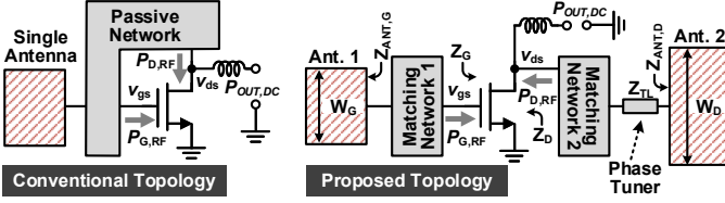
Fig. 5. Comparison between the conventional single-antenna topology and our dual-antenna topology.
