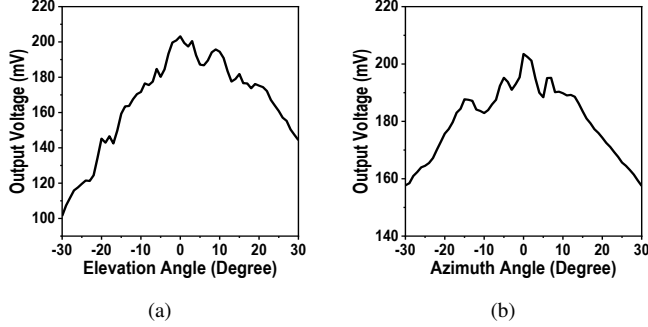
Fig. 9. Measured angle sensitivity in (a) E- and (b) H-planes.
