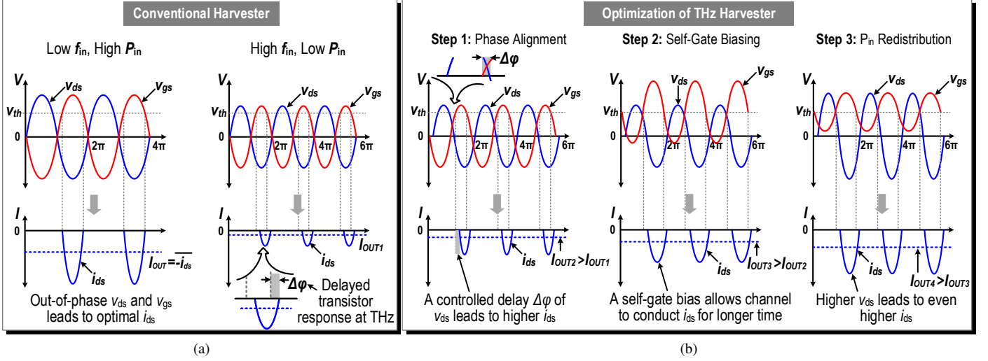
Fig. 3. Rectifying operation of FET in (a) a conventional harvester and (b) our THz harvester with step-by-step optimizations.
