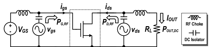
Fig. 2. A generalized testbench for rectification performance test.
