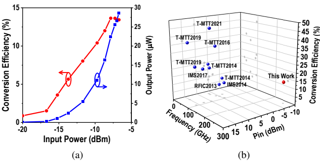
Fig. 10. (a) Measured \eta and P_{OUT,DC} with 1-k \Omega load. (b) Comparison of this work with the state-of-art mm-Wave energy harvesters.
