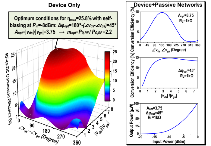
Fig. 4. Simulated rectification performance of a N-FinFET (8x270nm/22nm) at various v_{ds} and v_{gs} ratio and phase difference. The inset shows the simulated results including the losses from device vias and matching networks.
