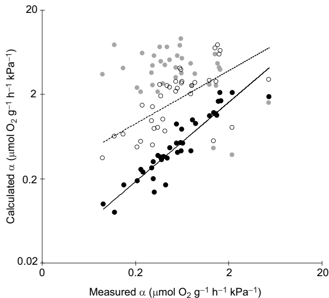
Fig. 4. The measured ( \alpha -method) and calculated (published \text{MR}/P_{crit} ) oxygen supply capacity ( \alpha ). Values are presented in Table S1. The measured \alpha (x-axis) is strongly correlated with that determined as \text{MR}/P_{crit} (y-axis) using reported values (black symbols, y = 1.07x - 0.10 ; Pearson's R = 0.96 , P < 0.001 ). Oxygen supply capacity is significantly correlated with MR ( \alpha = 0.195 \times \text{SMR} + 0.317 ; Pearson's r = 0.98 , P < 0.001 ; open symbols), but not the reported P_{crit} value (Pearson's r = -0.10 , P = 1 ; gray symbols). Data from Behrens and Steffensen, 2007; Birk et al., 2018; Birk et al., 2019; Brill et al., 2015; Burggren et al., 2019a,b; Caposella 2012; Childress, 1975; Childress and Seibel, 1998; Christensen and Colacino 2000; Claireaux and Chabot 2016; Collins et al., 2013; Cowles and Childress, 1995; Crear and Forteach, 2000; Dall 1986; Ern et al., 2016; Fu et al., 2011; Lefevre et al., 2015; Mandic et al., 2020; Negrete and Esbaugh, 2019; Nilsson and Ostlund-Nilsson, 2004; Onthank et al., 2021; Paschke et al., 2010; Reemeyer and Rees, 2019; Rutherford and Thuesen, 2005; Schurmann and Steffensen, 1997; Seibel and Childress, 2000; Slesinger et al., 2019; Snyder et al., 2016; Speers-Roesch, 2012; Staples et al., 2000; Stoffels 2015; Thuy et al., 2010; Tuong et al., 2018; Ultsch et al., 1981; Wishner et al., 2018.
