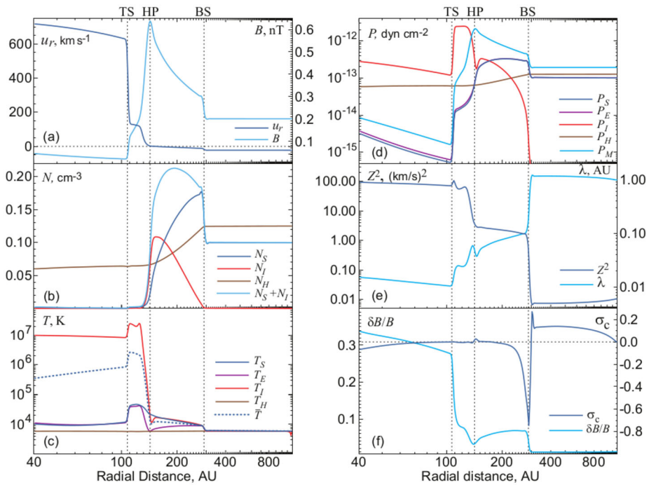
Fig. 8 Radial profiles of the flow, magnetic field, and turbulence parameters along the VI trajectory for the 0°-model from 40 AU to 1200 AU: (a) radial velocity u_r and magnetic field strength; (b) thermal proton N_S , pickup proton N_I , interstellar hydrogen N_H , and total proton N_S + N_I densities; (c) proton T_S , electron T_E , pickup proton T_I , interstellar hydrogen T_H , and mean \bar{T} temperatures, where \bar{T} = (T_S N_S + T_E N_E + T_I N_I) / (N_S + N_E + N_I) ; (d) proton P_S , electron P_E , pickup proton P_I , interstellar hydrogen P_H , and magnetic P_M pressures; (e) turbulent energy density Z^2 and correlation length \lambda ; (f) cross helicity \sigma_c and relative amplitude of the magnetic field fluctuations \delta B/B . The vertical lines mark the locations of the HTS, HP, and BS at \approx 105/140/290 AU, respectively. Reproduced from Usmanov et al. (2016)
