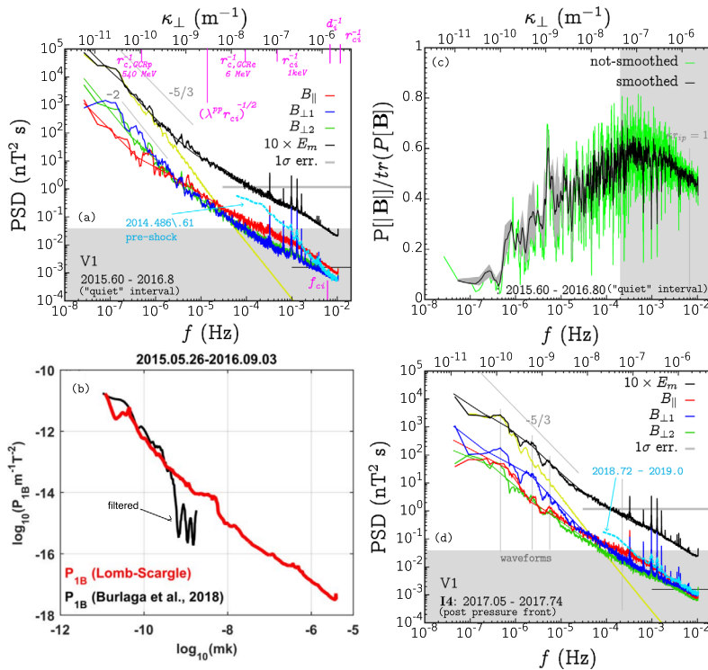
Fig. 27 Magnetic field spectra in the VLISM from VI data during a quiet interval (panels a , b , and c ) and during a post-shock interval (panel d ). Panel ( c ) shows the scale-dependent magnetic compressibility. Some relevant scales are reported in panel ( a ). Adapted from Fraternali and Pogorelov (2021), Lee and Lee (2020)
