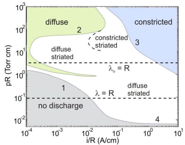
Figure 1. Discharge forms in neon for different discharge currents i and gas pressures p . Reproduced from [28]. © IOP Publishing Ltd. All rights reserved.
