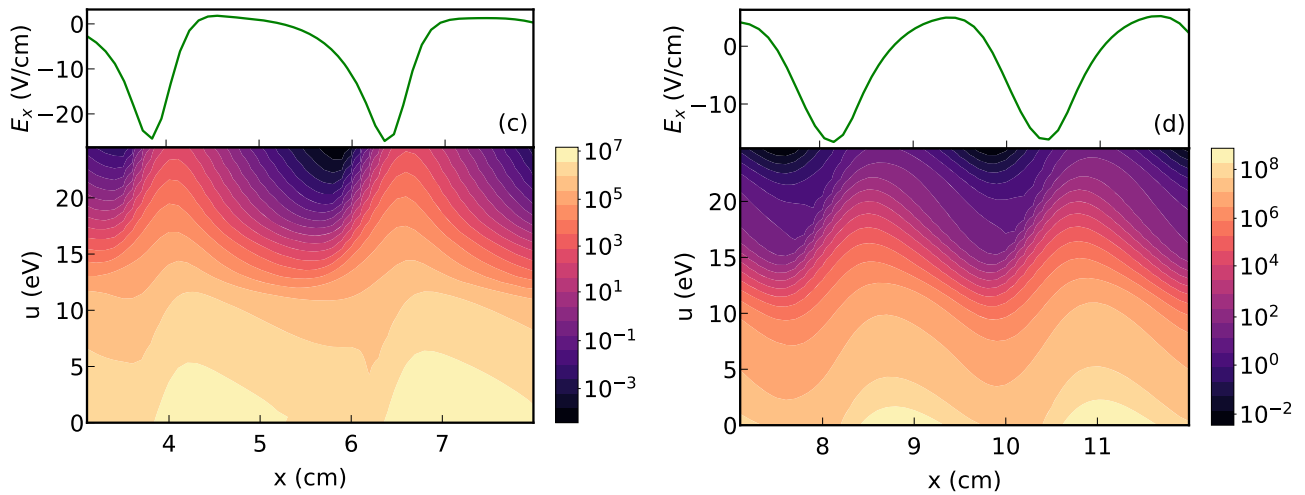
Figure 5. Instantaneous EEDFs for s -striations (left) and p striations (right) and the corresponding electric field profiles. Reproduced from [32]. © IOP Publishing Ltd. All rights reserved.
