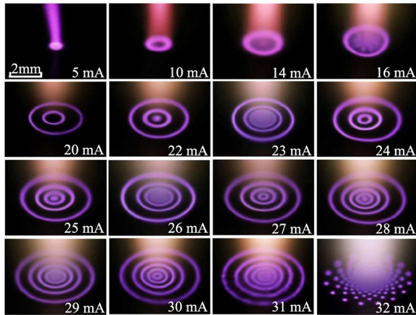
Figure 9. Anode patterns with increasing discharge current. DC discharge in the air with liquid waver anode gap width of 5 mm and exposure time of 100 ms. Reproduced from [64]. © IOP Publishing Ltd. All rights reserved.
