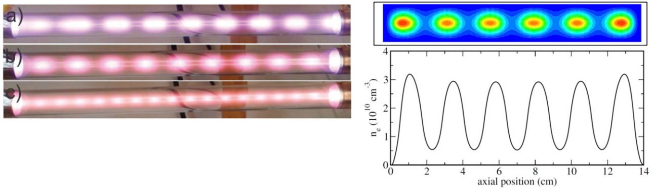
Figure 4. Experimental observation of standing striations in argon CCP at 3.6 MHz at pressure p = 0.1, 1 , and 10 Torr (left), and spatial distributions of electron density obtained in 2D simulations at 20 MHz (right). Reproduced from [31]. © IOP Publishing Ltd. All rights reserved.
