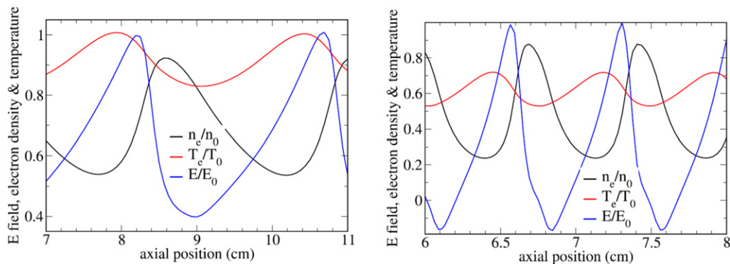
Figure 3. Axial distributions of the normalized electric field, electron density, and temperature for moving striations in the diffuse (left) and constricted (right) discharges at high currents. Reprinted from [30], with the permission of AIP Publishing.
