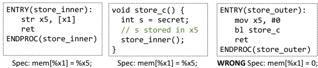
Figure 5: An example of incorrectly combining C and assembly specifications. Assembly function store_outter clears register x5 to 0, then calls C function store_c . store_c calls assembly function store_innner , which stores register x5 into memory. The intended behavior is that the value 0 will be stored to memory. The actual behavior is that x5 stores C temporary variable s which contains secret data, resulting in undetected information leakage.
