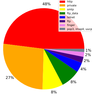
(a) KDD99
