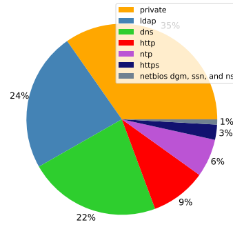
(e) CUPID
