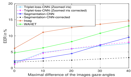
Fig. 5: Recognition results (EER in%) for the triplet loss CNN approach (with and without gaze angle correction) and the comparison approaches for an increasing maximum gaze angle difference between images
