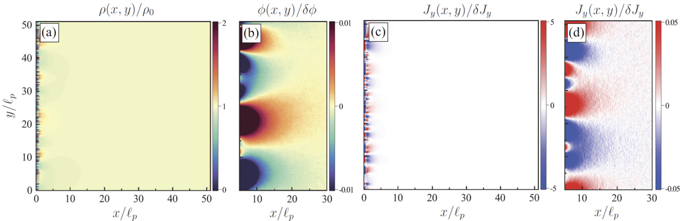
FIG. 2. Steady-state density and currents for run-and-tumble particles on a lattice, in the presence of a disordered wall at x = 0 and periodic boundary conditions along the \hat{y} direction. The disordered wall is modeled as a random potential which vanishes for x larger than the particle persistence length \ell_p ; for other numerical details, see Appendix A. (a) Particle density \rho(x, y) in the full system, normalized by the average density. Lengths are rescaled by the particle run length \ell_p . Note the presence of a strong density accumulation close to the wall at x = 0 that is modulated by the disorder. The color code corresponds to \rho(x, y)/\rho_0 . (b) Density modulation \phi(x, y) \equiv \rho(x, y) - \langle \rho(x) \rangle in the bulk of the system, where \langle \rho(x) \rangle is the average density at a distance x from the wall, normalized by the standard deviation of the density modulation \delta\phi . The density modulations extend deep in the bulk of the system, far beyond the microscopic scales set by the particle run length and the disordered wall. (Note that the x axis starts at five run lengths from the wall.) (c) Current along the \hat{y} direction in the full system, normalized by the current standard deviation \delta J_y . At this scale, a localized current flowing along the wall is observed, as expected from the existing literature [36]. (d) A close-up on the bulk region shown in panel (b) reveals the existence of large eddies whose scales increase with the distance from the wall.
