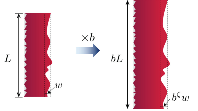
FIG. 8. An illustration of the scaling procedure used to construct the Imry-Ma argument. As the system size is increased by a factor of b , the width of the interface between the phases is multiplied by b^\zeta . The interface is well defined in the large system-size limit when \zeta < 1 .
