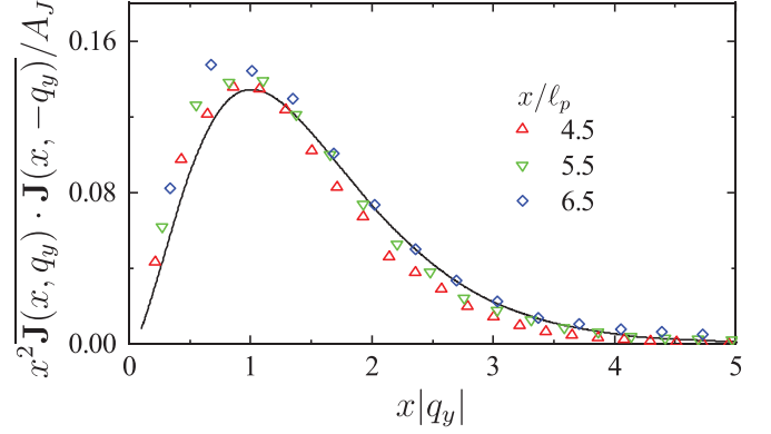
FIG. 5. Fourier transform along the \hat{\mathbf{y}} direction of the current-current correlation function measured at a distance x from the wall and averaged over disorder. The data are measured for three values of x and normalized by a factor A_J \equiv 2d(2\pi)^{d-1}(\mu\sigma p)^2 . As predicted by our theory, the data can be collapsed onto a single curve, corresponding to Eq. (30), by properly scaling the abscissa and the ordinates. See Appendix A for numerical details.
