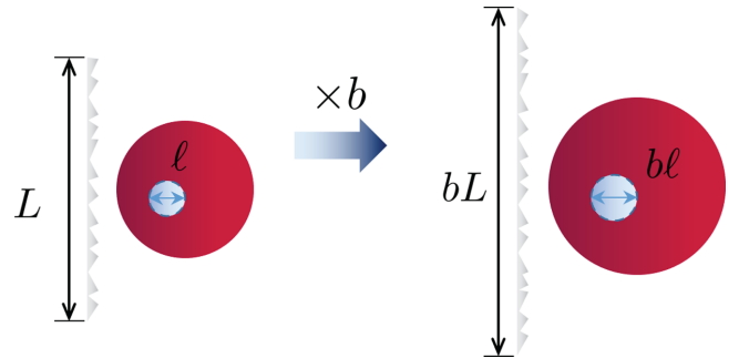
FIG. 11. The scaling argument presented in Fig. 9 for the wetting layer can be adapted to the case of a liquid droplet. Upon scaling the system size by a factor of b , we compare the scaling of the bulk and surface energies, whose competition determines if the droplet is macroscopically stable.
