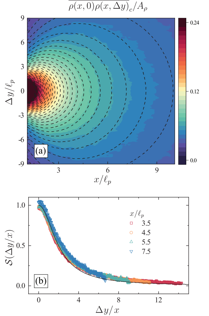
FIG. 4. Disorder-averaged two-point density correlation function of noninteracting RTPs in two dimensions in the presence of a disordered wall at x = 0 . (a) The two-point correlation function as x and \Delta y are varied, calculated from simulations, is shown by the color map. The value of A_\rho \equiv \ell_p S_d^{-1} (2\mu p \sigma / \mathcal{D}_{\text{eff}})^2 is obtained from a fit of the data to Eq. (25). The latter includes a constant offset due to finite-size corrections, which is calculated exactly in Appendix C. The theoretical prediction of Eq. (25) is then used to produce dashed contour lines that match the levels of the color bar. Both theory and simulations are normalized by A_\rho . (b) A verification of the scaling form (26) for the density-density correlation function. The data shown in panel (a) for four different distances x from the wall are collapsed onto a single curve, as predicted. See Appendix A for numerical details.
