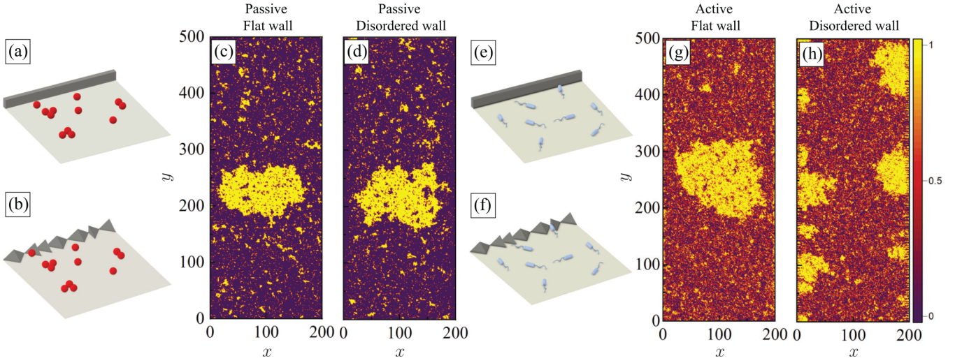
FIG. 1. Impact of flat (a), (e) and disordered walls (b), (f) on phase separation in passive (a), (b) and active (e), (f) systems. In the presence of attractive interactions, simulations of a passive lattice gas at low temperature shows phase separation in both settings (c), (d). In contrast, simulations of an active lattice gas (h) show that the disordered boundary destroys the phase separation observed in the presence of a flat wall (g). Color encodes density; see Appendix A for further numerical details.
