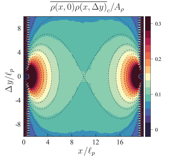
FIG. 6. Disorder-averaged two-point density correlation function of noninteracting RTPs measured in the presence of two disordered walls at x = 0 and x = 20\ell_p . Periodic boundary conditions are imposed along the \hat{\mathbf{y}} direction. The correlation function is normalized by a factor A_\rho \equiv \ell_p S_d^{-1} (2\mu p \sigma / D_{\text{eff}})^2 . Simulation results are shown as a color map and compared to the analytic predictions of Eq. (D2) (dashed contour lines). See Appendix A for numerical details.
