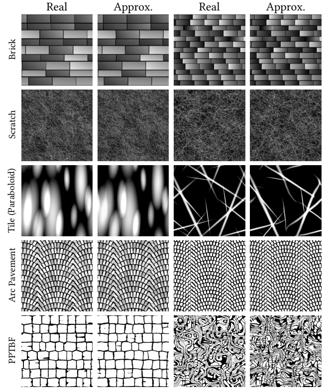
Figure 5: We compare generator maps synthesized by our proxies (Approx.) with their original procedural counterpart (Real) via randomly sampled parameters, showing that they are very close. See supplemental documents for results generated from all our trained proxies.
