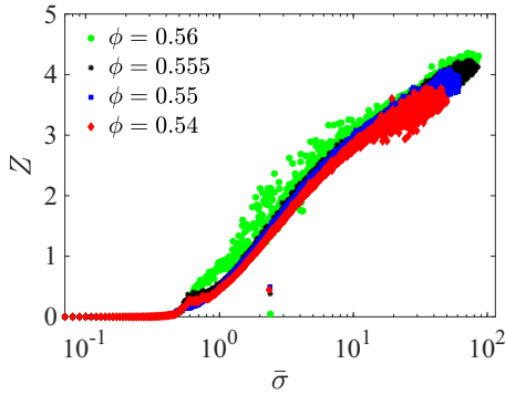
FIG. 5. Frictional contact network degree Z , as a function of suspension shear stress, \bar{\sigma} for \phi = 0.54, 0.55, 0.555 , and 0.56 . Each point represents a time sample, and the full range of shear rate \dot{\gamma} is represented. The change in slope at Z \approx 0.28 is shown later to correspond to contact percolation.
