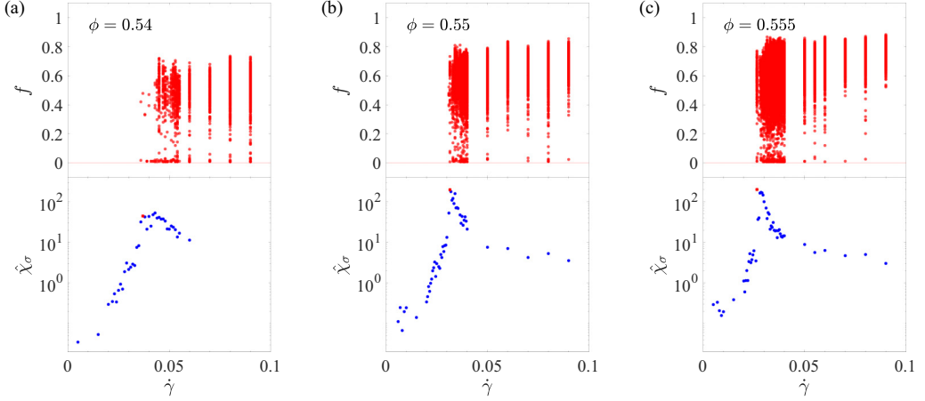
FIG. 16. Fraction of 3-cores (top) and stress susceptibility (bottom) as a function of shear rate, for (a) \phi = 0.54 , (b) \phi = 0.55 , and (c) \phi = 0.555 . The red point in each stress susceptibility plot at bottom corresponds to the first appearance of a 3-core.
