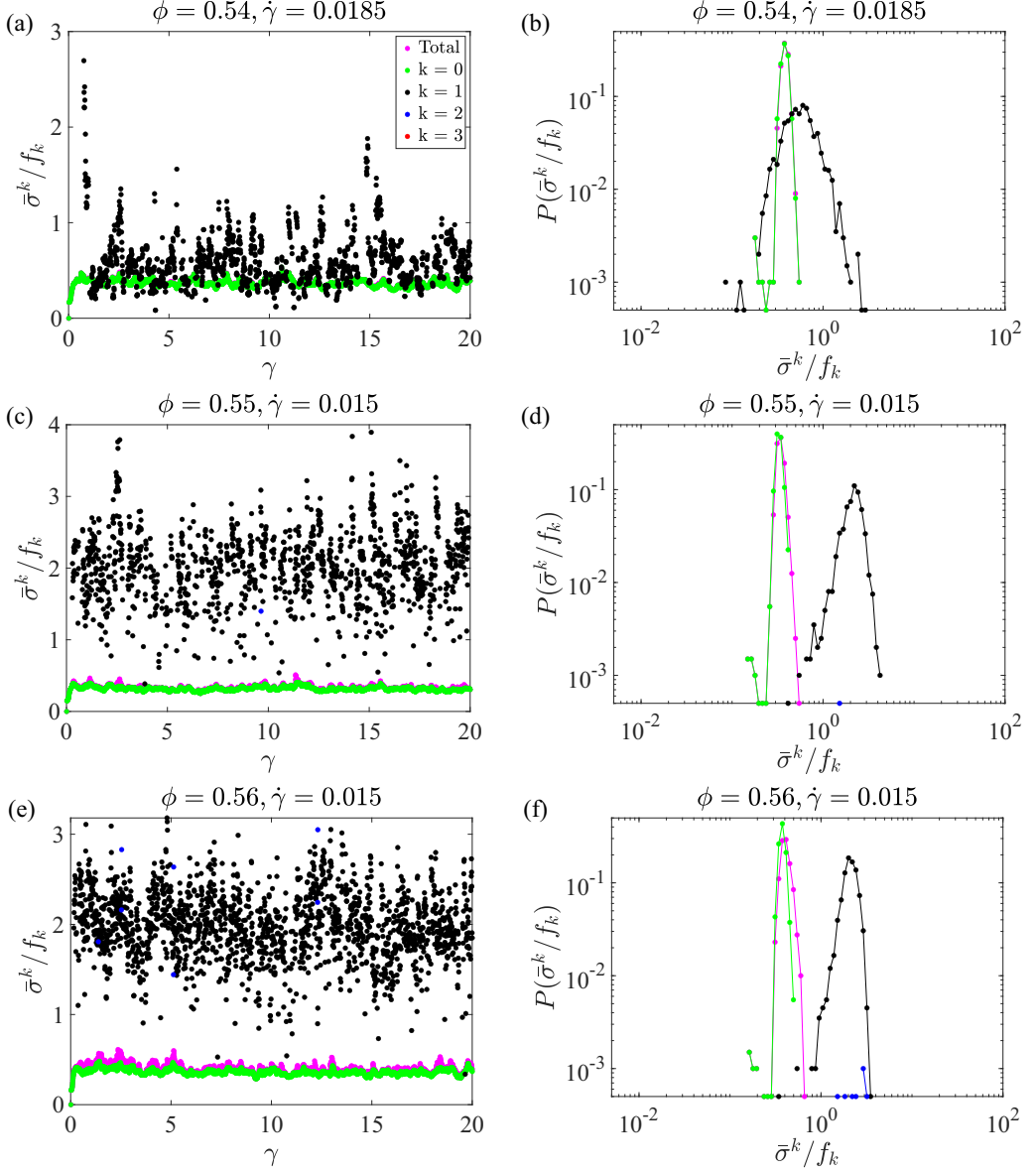
FIG. 17. Core-averaged stress as a function of strain (left) and its distribution (right) at the onset of shear thickening (a), (b) \phi = 0.54 and \dot{\gamma} = 0.0185 , (c), (d) \phi = 0.55 and \dot{\gamma} = 0.015 , and (e), (f) \phi = 0.56 and \dot{\gamma} = 0.015 . Legend in part (a) applies to all plots. Note that no 3-cores (red points) are present and only very few 2-cores (blue points).
