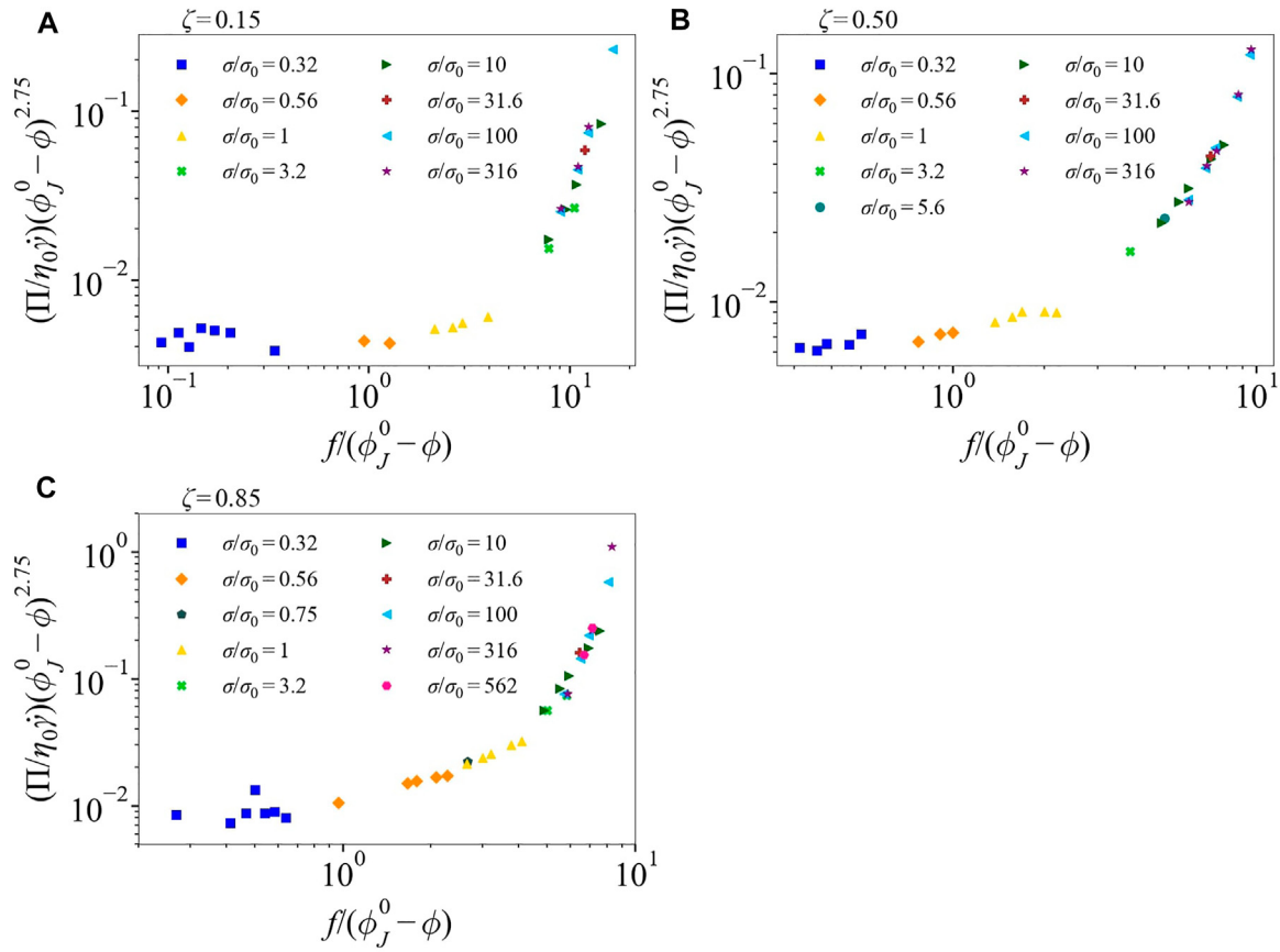
FIGURE 6 | The scaling function \mathcal{F}_{\Pi} = \hat{\Pi}(\phi_J^0 - \phi)^{2.75} (note the different exponent relative to \mathcal{F}_{\eta} and \mathcal{F}_{N_2} in the prior two figure) plotted as a function of the scaling variable x = f/(\phi_J^0 - \phi) for bidisperse suspensions at \delta = 3 and varying large particle fraction (A) \zeta = 0.15 (B) \zeta = 0.50 , (C) \zeta = 0.85 over 0.54 \leq \phi \leq 0.60 and 0.32 \leq \sigma/\sigma_0 \leq 562 . For \zeta = 0.15 , the form of f is exponential f(\sigma) = \exp(\sigma^*/\sigma) with \sigma^* = 1.45 ; for \zeta = 0.50 and 0.85 , it is fitted manually f = f_{\text{fit}} .
