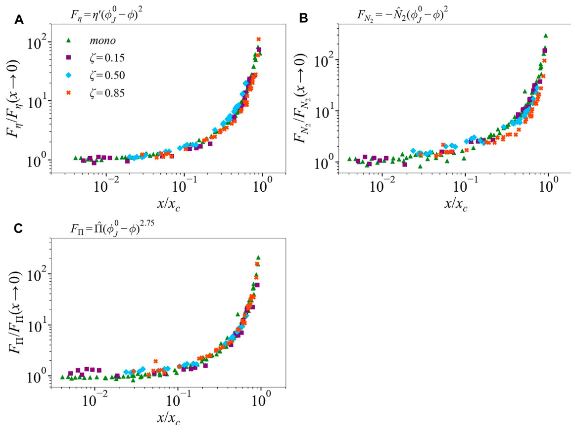
FIGURE 8 | Scaling functions (A) \mathcal{F}_\eta , (B) \mathcal{F}_{N_2} , and (C) \mathcal{F}_\Pi , normalized by their baseline values, versus the scaling variable x/x_c for simulated monodisperse ( \delta = 1.4 and \zeta = 0.50 over 0.52 \leq \phi \leq 0.63 ) and bidisperse ( \delta = 3 for \zeta = 0.15, 0.50, 0.85 over 0.54 \leq \phi \leq 0.60 ) suspensions, where x = f/(\phi_J^0 - \phi) and x_c = 1/(\phi_J^0 - \phi_J^*) . For monodisperse suspension and bidisperse suspension at \zeta = 0.15 the form of f is f(\sigma) = e^{-\sigma/\sigma_0} . For bidisperse suspensions at \zeta = 0.50 and 0.85 it is f_{\text{fit}} . The legend in panel (A) is used in all plots.
