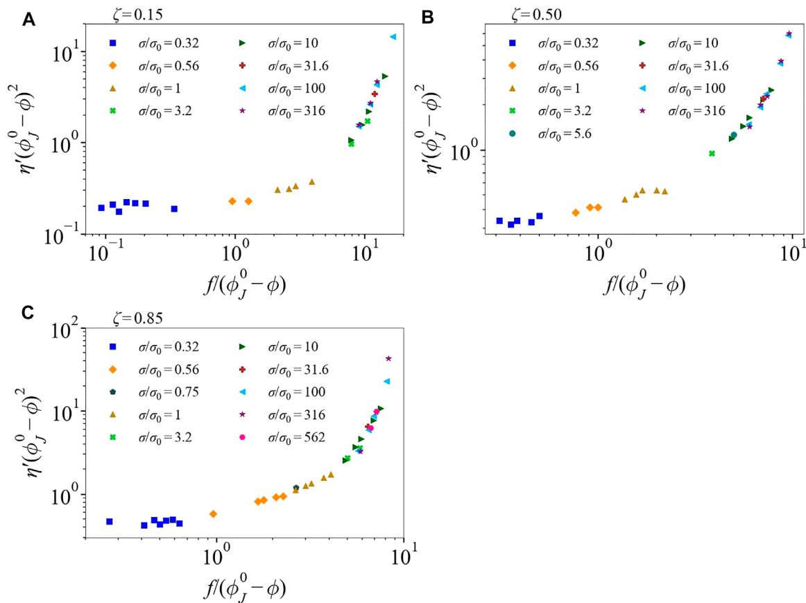
FIGURE 4 | The scaling function \mathcal{F}_\eta = \eta'(\phi_J^0 - \phi)^2 plotted as a function of the scaling variable x = f(\phi_0 - \phi) for bidisperse suspensions at \delta = 3 and varying large particle fraction (A) \zeta = 0.15 (B) \zeta = 0.50 , (C) \zeta = 0.85 over 0.54 \leq \phi \leq 0.60 and 0.32 \leq \sigma/\sigma_0 \leq 562 . For \zeta = 0.15 , the form of f is exponential f(\sigma) = \exp(\sigma^*/\sigma) with \sigma^* = 1.45 , for \zeta = 0.50 and 0.85 , it is fitted manually f = f_{\text{fit}} .
