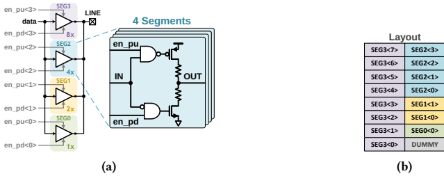
Figure 5: A line driver design with array structure. (a) The schematic. (b) Manual layout abstraction.
