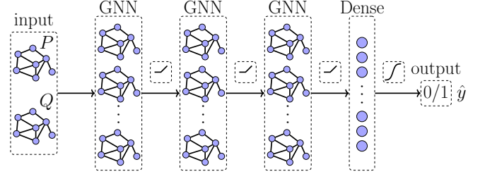
Fig. 3. Architecture of the proposed GNN based detector.
