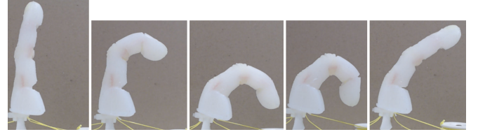
Fig. 9. Poses illustrating the range of motion of a four-cable hybrid soft-rigid robotic finger.
