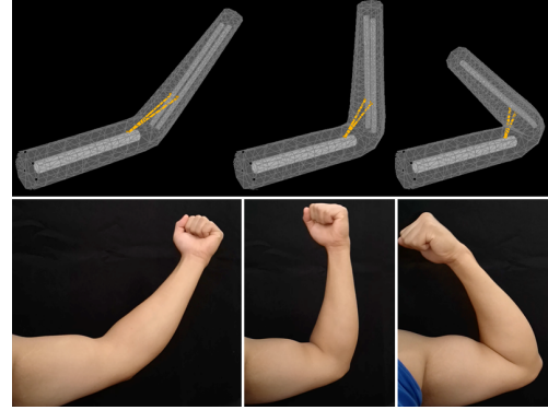
Fig. 12. An exploratory simulation of a 3D bio-inspired hybrid soft-rigid robotic arm with nonplanar skeleton. The top row shows the simulations corresponding to the bottom poses of a human arm.
