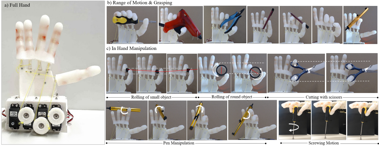
Fig. 10. The full hybrid soft-rigid hand (a) is capable of grasping various objects and performing simple in-hand manipulation tasks. (b) shows the range of grasps that can be achieved with (c) highlighting some of the in-hand manipulation tasks.
