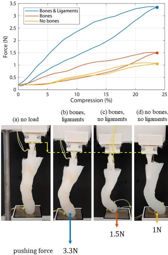
Fig. 7. We show that the addition of bones and ligaments can enable a robot to apply greater force. To demonstrate this we bolt the base of a soft finger into a linear stage, and position a force sensitive resistor (FSR) below it. We drive the finger down (and then back up), and plot the force measured by the FSR. We repeat this procedure for three conditions. Snapshots are shown in the pictures below, with corresponding dots drawn on the plot.
