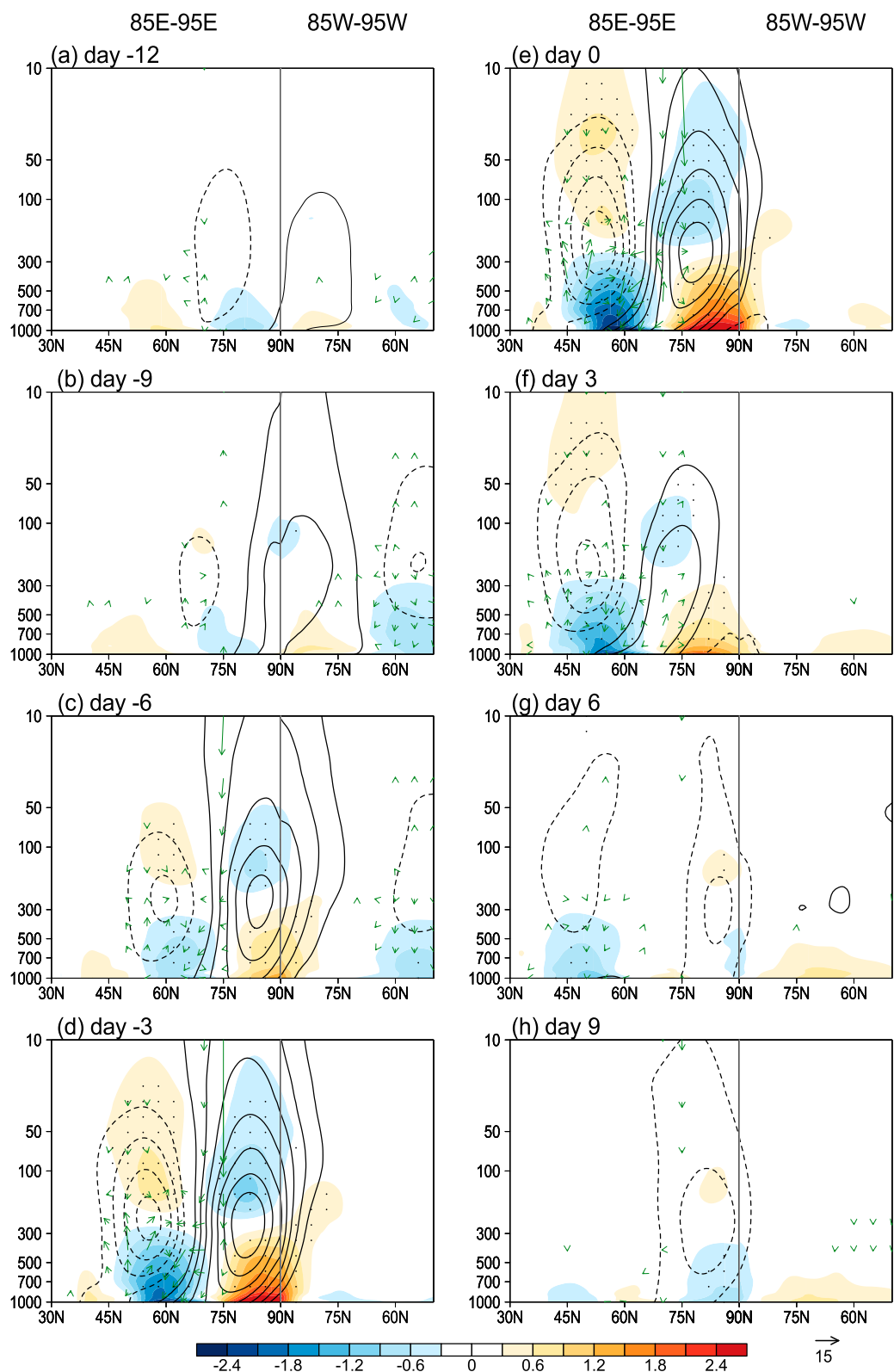
FIG. 10. As in Fig. 5, but based on ECHAM AGCM simulations.
