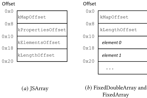
Figure 2: JavaScript object layouts in V8
