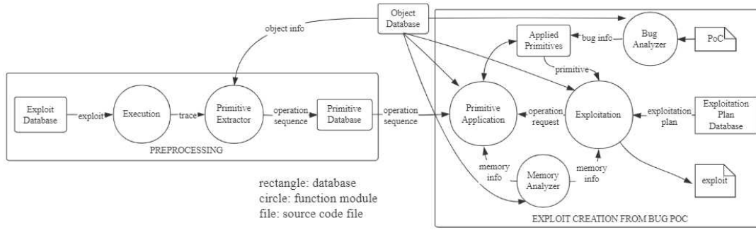
Figure 1: Automatic Exploit Generation Framework
