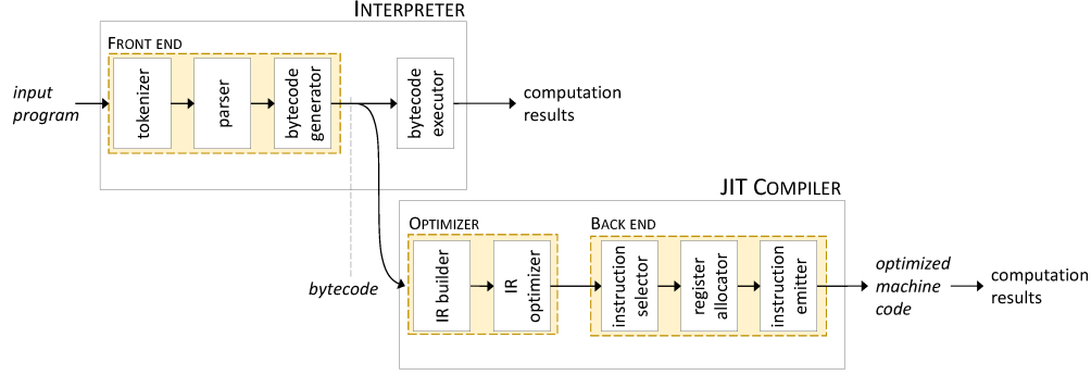
Figure 1. Interpreter/JIT Compiler Systems: Organization and structure
