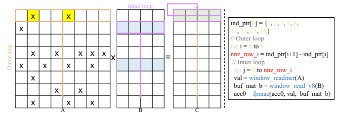
Fig. 5. Row-wise sparse-dense matrix multiplication.
