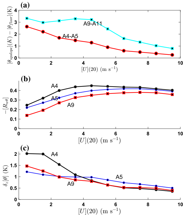
Fig. 6 The dependence on the wind speed U (20 m) for mostly clear conditions ( R_{\text{net}} < -40 \text{ W m}^{-2} ) for a the two-point temperature differences [\theta_{\text{upslope}}] - [\theta_{\text{floor}}] ; b the correlation coefficient [R_{w\theta}] ; and c \delta_z[\theta] . The measurements include station A5 (blue circles) on the gully floor, station A4 (black asterisks) upslope from the gully floor, station A11 on the valley floor and station A9 (red squares) upslope from the main valley floor. For locations, see Fig. 1
