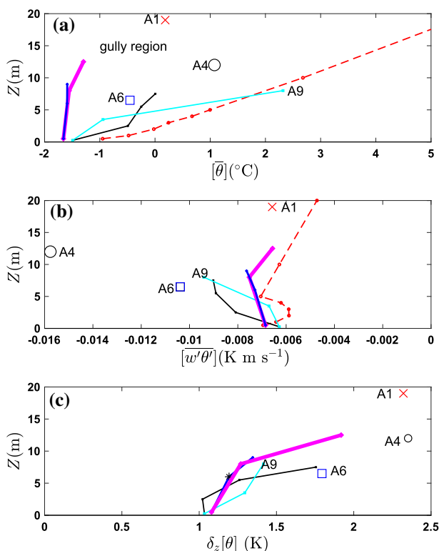
Fig. 2 Spatial variation of a [\theta] , b [w'\theta'] , and c \delta_z[\theta] , for very stable cases where U ( 20 \text{ m} ) < 3 \text{ m s}^{-1} and [\langle \delta_z \theta \rangle] > 1 \text{ K} . Transects are located in the south gully (thick blue line) and in the north gully (thick magenta line). Individual stations emphasized in the upland gully region are station A1 at the edge of the western plateau (red X), A6 between the gullies (blue square), and station A4 north of the north gully (black circle) (Fig. 1). Included for reference is the tower profile in the main valley (thin red dashed), the transect on the south shoulder of the main valley (thin black), and on the north shoulder (thin cyan). The height Z is with respect to the base of the main tower
