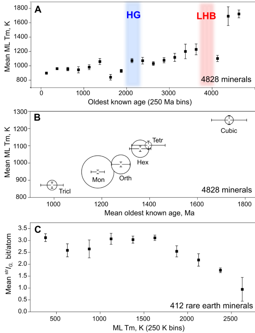
Figure 3. Machine learned melting temperature (ML Tm) for minerals from RRUFF dataset A ) Mean ML Tm vs. oldest known age. The highlights correspond to the timing of hypothesized Late Heavy Bombardment (LHB) and Huronian Glaciation (HG) events. B ) ML Tm vs. oldest known age for all minerals grouped by crystal systems. The size of the circles scaled with the number of minerals: (cubic: 500; tetragonal: 383; hexagonal: 855; orthorhombic: 932; monoclinic: 1600; triclinic: 509. C ) Mean structural complexity index vs. predicted melting temperature for 412 rare earth containing minerals. The error bars correspond to standard errors.
