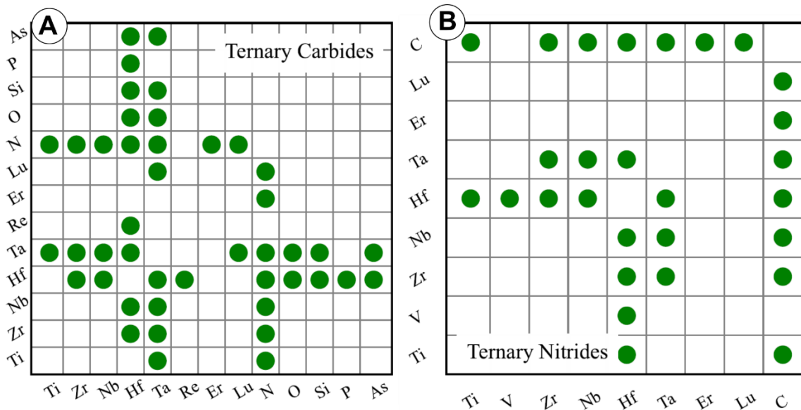
Figure 4. Constituent elements in ternary carbides (A) and nitrides (B) with predicted melting temperatures above 3500 K. Each dot represents one ternary compound, M1-M2-C, or M1-M2-N with M1 and M2 being the corresponding elements on the axes.
