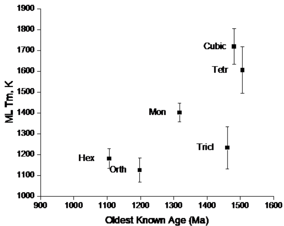
Fig. S2. Predicted melting temperature 1 vs. oldest known age for 401 rare earth containing minerals from RRUFF dataset ( https://rruff.info/ima/ ) 2,3 , averaged by crystal system (cubic: 21; tetragonal: 23; orthorhombic: 80; hexagonal: 112, monoclinic: 138). Melting temperature model was built based on a dataset of 9375 compounds.
