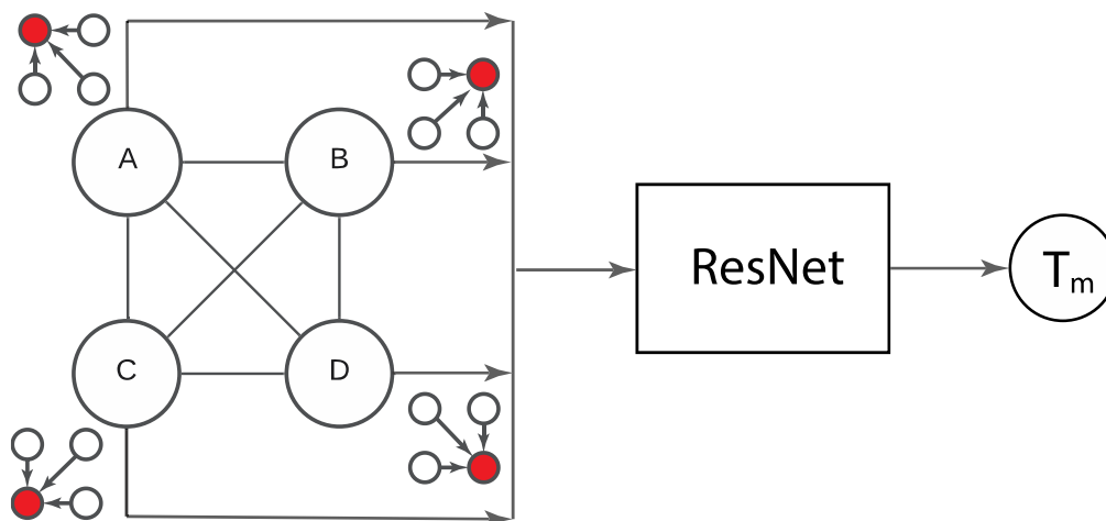
Figure 1. Architecture of the GNN model for ML melting temperature prediction. Each circle represents an element and its composition in the material. Up to four elements are connected in this graph (denoted as A, B, C, and D). First, each element and composition are converted to 14 features, which are then encoded and fed to the ResNet input layer. The circles communicate with each other in order to account for higher order contributions. For example, each circle (element and composition) pulls information from other circles via the GNN. The outputs are then sent to the ResNet. The latter consists of four fully connected layers with skipping connections and leads to the regression analysis for melting temperature prediction
