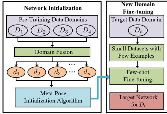
Fig. 2. Illustrate the training procedure of Meta-Pose.
