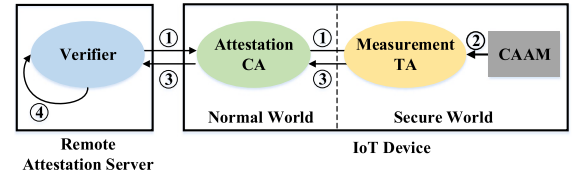
Fig. 5. Remote attestation process.
