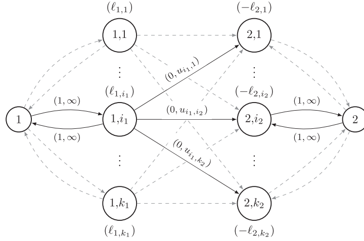
Fig. 1. MCNF graph corresponding to formulation (3). Arc labels have the form (cost, upper bound), and non-zero supplies and demands are displayed next to each node.
