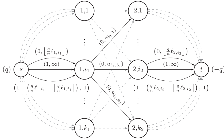
Fig. 3. MCNF graph for formulation (7). Arc labels have the form (cost, upper bound), and non-zero supplies and demands are displayed next to each node. Costs displayed in the figure omit a 2/q scaling.
