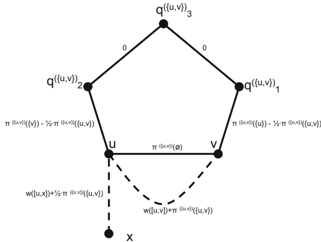
Fig. 1 An example of the graph \tilde{G} where G has three nodes x, u, v and two edges [x, u], [u, v] and P consists of one pair \{u, v\} . The dashed edges are edges in E whereas the solid edges are in E_{\{u, v\}} . Next to each edge we state its weight according to w'
