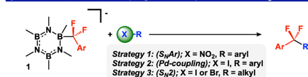
Figure 1. a) Bioactive compounds with an \text{ArCF}_2\text{--R} motifs. b) Previous work: cross-coupling reactions of aryl and alkyl \text{CF}_2\text{X} . c) This work: nucleophilic strategies to form C–C CF bonds.
