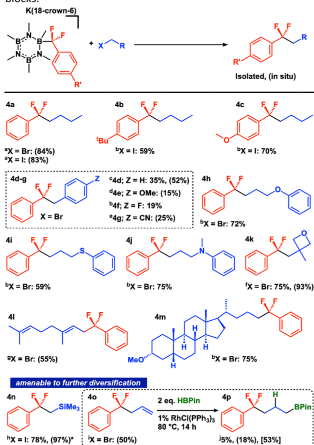
Figure 3. S N 2 reactions with alkyl halides. In situ yields measured by 19 F NMR with respect to an internal standard, PhOCF 3 or PhF. a 1 eq. [B]CF 2 Ar (0.02 mmol), 1.2 eq. RCH 2 X, 90 °C, 30 min in toluene (0.02M). b 1.5 eq. [B]CF 2 Ar, 1 eq. RCH 2 X (0.25 mmol), 90 °C, 12 h in toluene (0.02M). c 1 eq. [B]CF 2 Ar (0.3 mmol), 1.2 eq. RCH 2 X, 80 °C, 18 h in THF (0.02M). d Same as c but on a 0.01 mmol scale. e Same as b but on a 0.1 mmol scale. f 1 eq. [B]CF 2 Ar (0.3 mmol), 1.2 eq. RCH 2 X, 25 °C, 18 h in THF (0.02M). g 1 eq. [B]CF 2 Ar (0.15 mmol), 1.5 eq. RCH 2 X, 23 °C, 12 h in toluene (0.02M). h Same as f but on a 0.1 mmol scale. i Same as f but stopped after 3.5 h. j After formation of 4o , solids removed by filtration and allyl bromide removed by vacuum. 4p heated to 80 °C in 15 mL THF in the presence of pinacol borane (2eq.) and RhCl(PPh 3 ) 3 for 14 h. Yields for 4p were determined over two steps. * isolated in 1:1 mixture with hexamethylborazine. [selectivity for product].
