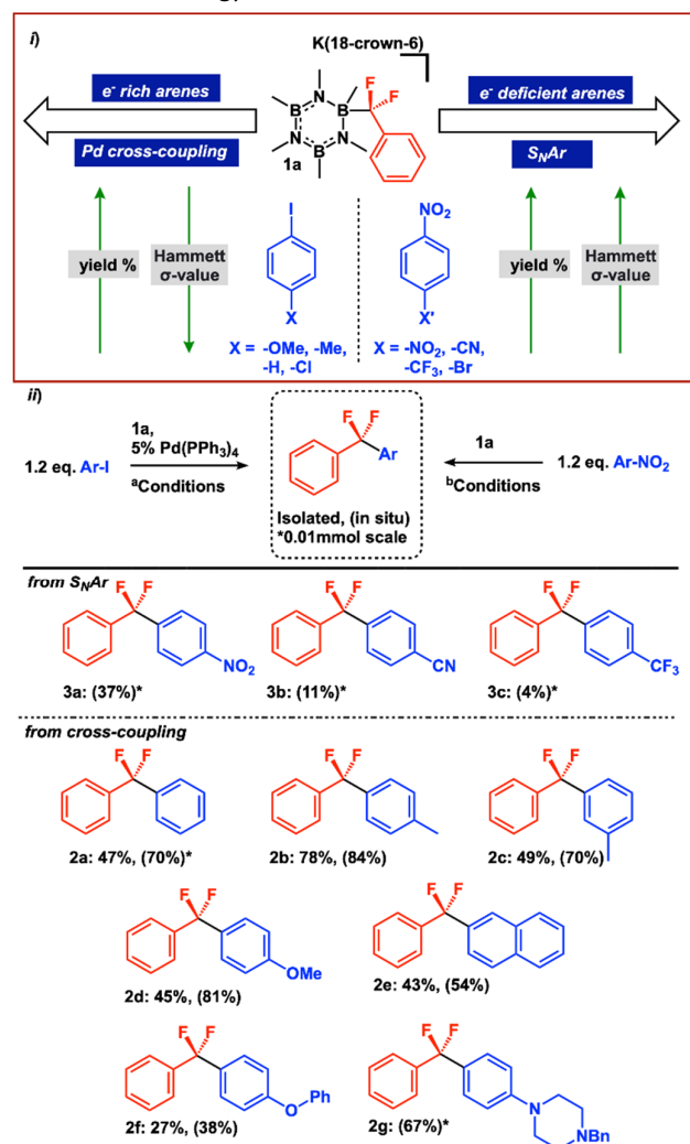
Figure 2. i) Electronic trends with Pd catalyzed cross-coupling and S N Ar. ii) Scope in cross coupling and S N Ar. In situ yields measured by 19 F NMR with respect to an internal standard, trifluoromethyl anisole. Mass purity of isolated samples measured by 19 F NMR with respect to an internal standard, trifluoromethyl anisole. a Conditions: reactions performed in toluene (0.02M) at 25 °C, 16h with 5 mol% Pd(PPh 3 ) 4 . b Conditions: reactions performed in THF (0.02M) at 25 °C, 18h.
