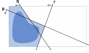
Fig. 2. Example space where ite(p, r, q \wedge r) \leq r .
