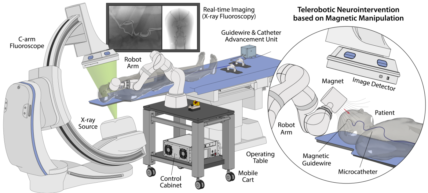
Figure 1. Overview of the telerobotic neurointerventional platform based on magnetic manipulation. The system features a light-weight, compact robot arm with an actuating magnet attached to its end-effector to remotely control a magnetically steerable guidewire through spatial positioning of the magnet around the patient's head. Mounted on a mobile platform beside the operating table, the robot arm is teleoperated from a remote-control console to steer the magnetic guidewire under real-time fluoroscopic imaging. The system further integrates a guidewire/microcatheter advancing unit based on a pair of motorized linear drives that can advance or retract the guidewire and a microcatheter upon remote control.
