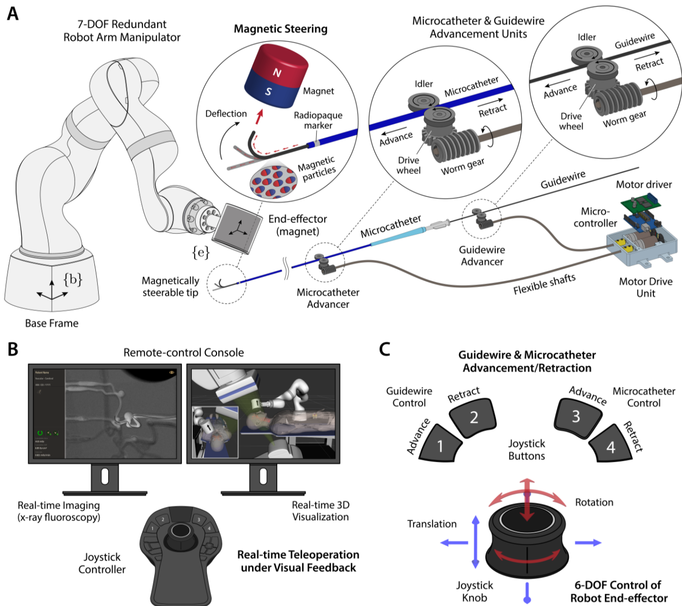
Figure 2. Description of the telerobotic neurointerventional system. (A) The robot arm has 7 degrees of freedom (DOF) with kinematic redundancy for flexible manipulation and safer operation in cluttered environments. The guidewire has a magnetically responsive tip that contains magnetic particles, and hence can be steered by the actuating magnet at the robot arm's end-effector. The guidewire is compatible with a standard microcatheter which travels over the guidewire along the navigated path. The guidewire and the microcatheter can be advanced/retracted by a pair of advancing units, each of which uses a worm drive to convert the rotary motion of the DC motor at the base to a linear motion. (B) The system is teleoperated from the remote-control console under feedback from real-time imaging of the guidewire/microcatheter in the blood vessels and virtual visualization of the robot arm. The magnetic guidewire is naturally visible under x-ray due to the embedded magnetic particles, and the position of the microcatheter can be identified by the radiopaque marker at the distal end. The robot arm is visualized in a virtual environment that replicates the real world on the control workstation to allow the operator to avoid collisions with surrounding objects while teleoperating the robot arm. (C) Spatial positioning of the magnet is achieved via 6-DOF position control of the robot arm's end-effector with a joystick controller, and advancement/retraction of the guidewire and the microcatheter can be controlled either independently or simultaneously with the joystick buttons.
