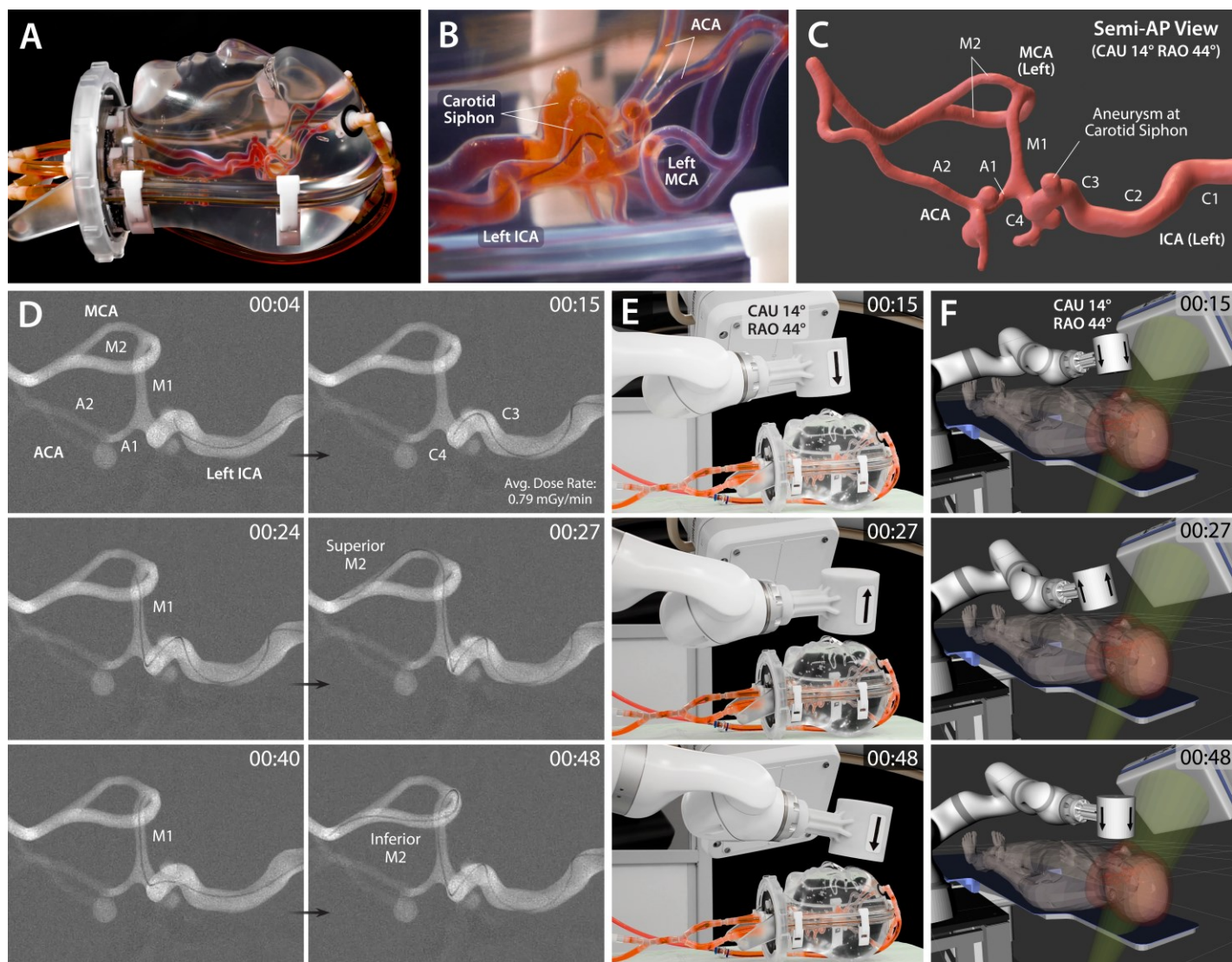
Figure 4. In vitro demonstration of magnetic steering and navigation in intracranial arteries under real-time x-ray fluoroscopy. (A) Realistic human head phantom with replicated intracranial arteries based on silicone vessels. (B) Lateral view of the magnetic guidewire navigating in the left ICA with its distal tip being directed toward the descending portion of the carotid siphon under repulsive steering to avoid contact with the aneurysm at the apex of the carotid siphon. (C) 3D model of the target vasculature viewed from a semi-anteroposterior (AP) projection which shows all the important anatomical landmarks including the carotid siphon with an aneurysm, the ICA bifurcation (A1-M1 junction), and the MCA bifurcation at the same time. (D) Fluoroscopic images of the magnetic guidewire navigating from the left ICA to MCA under telerobotically controlled magnetic steering to reach the superior and inferior M2 segments selectively in sequence. As part of the preprocedural step, digital subtraction angiography was performed to visualize the target vasculature as a roadmap for guidewire steering and navigation. ICA: internal carotid artery; MCA/ACA: middle/anterior cerebral artery. (E) Actual view and (F) virtual visualization of the robot arm with an actuating magnet, the C-arm providing the semi-AP projection for the target vasculature in caudal angulation of 14° (CAU 28°) and right anterior oblique rotation of 44° (RAO 44°), the human head phantom (or equivalently the virtual human patient) on the operating table. The arrow on the actuating magnet indicating the magnet's polarity identifies which steering mode is being used. A live fluoroscopy video is available in movie S2 , which also shows the robot motion under real-time teleoperation in both the physical and virtual environments. The average time it took for the demonstrated navigational task was 45.0 \pm 4.0 s ( n = 5 ) from 5 trials.
