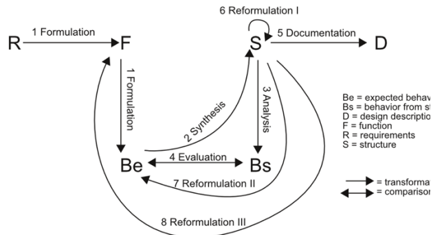
• FIGURE 1: FBS FRAMEWORK (SOURCE: [23, 24]).
