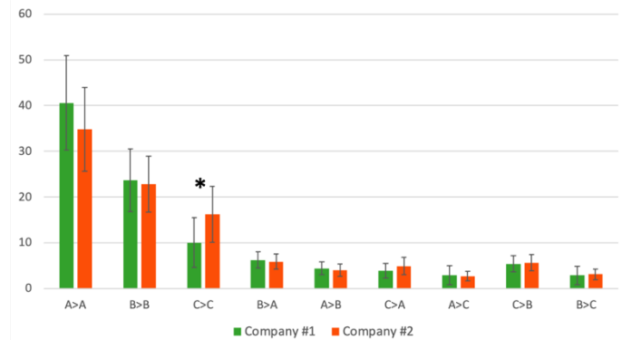
FIGURE 2: AVERAGE DISTRIBUTION OF TEAM MEMBERS' INTERACTIONS FOR TEAMS IN EACH COMPANY (* INDICATES STATISTICAL DIFFERENCES BETWEEN COHORTS)
