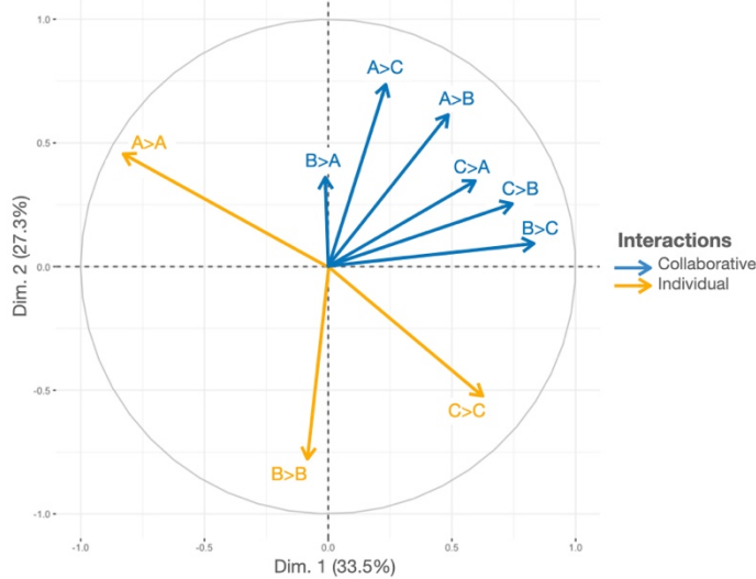
FIGURE 3: MULTIPLE FACTOR ANALYSIS CORRELATION CIRCLE OF QUATITATIVE VARIABLES: COLLABORATIVE FBS DESIGN PROCESSES (A>B, B>A, B>C, C>B, A>C, C>A) AND INDIVIDUAL FBS DESIGN PROCESSES (A>A, B>B, C>C)
