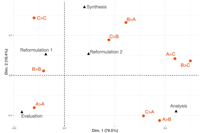
FIGURE 7: CORRESPONDANCE ANALYSIS ILLUSTRATING QUALITATIVE RELATIONSHIP BETWEEN INTERACTIONS AND FBS DESIGN PROCESSES FOR COMPANY #2
