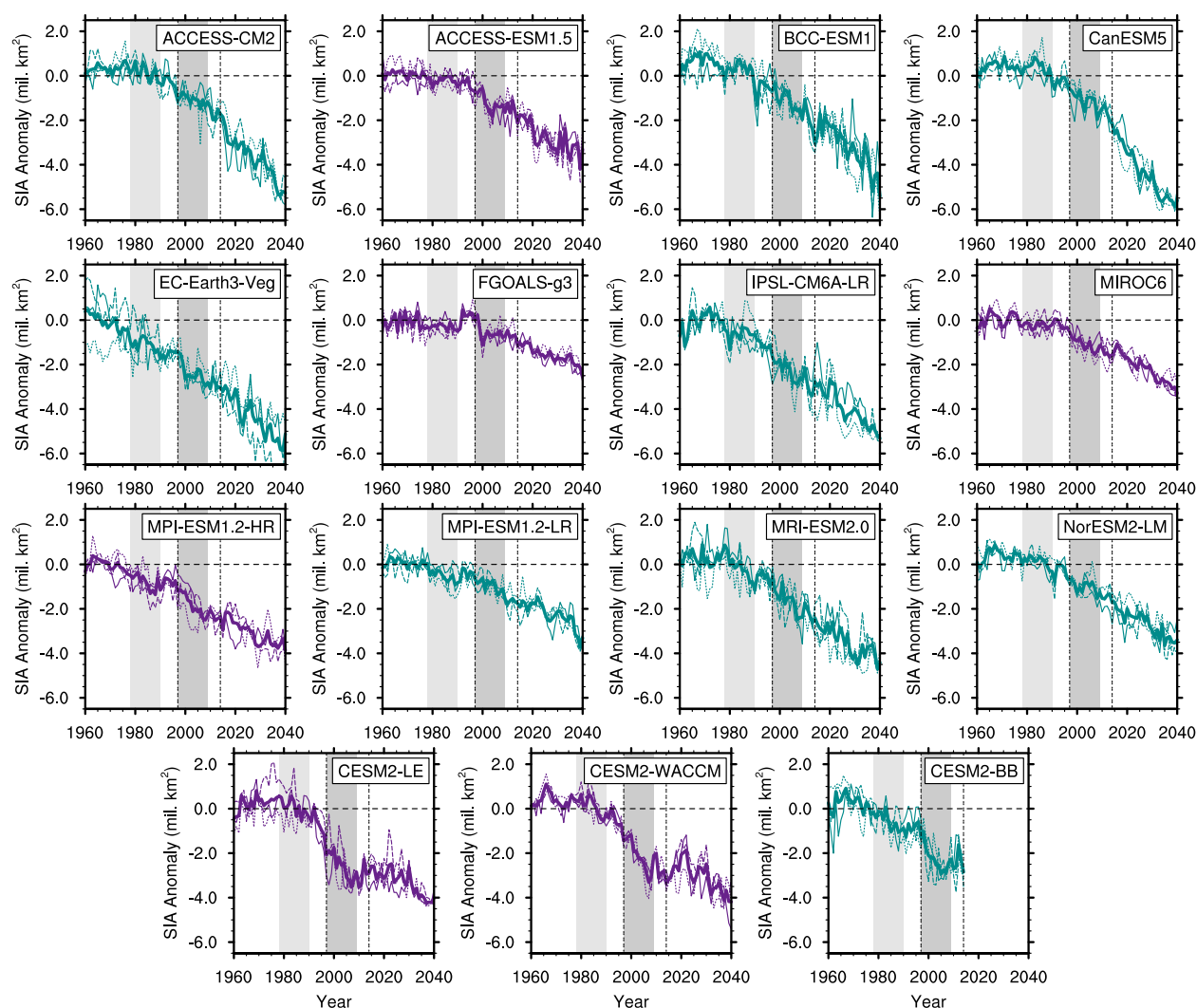
Fig. S6. September sea ice evolution in CMIP6 models. September sea ice area (SIA) anomalies relative to the 1940–1969 average for each CMIP6 model. Models in the sensitive category are shown in purple and the ones in the not sensitive category are shown in turquoise. For each model, the first three ensemble members are shown as thin lines and the ensemble mean is shown by the thick line. The light gray shaded region corresponds to the reference period 1978–1990 and the dark gray shaded region corresponds to the acceleration period 1997–2009 (see Materials and Methods for more details). The horizontal dashed line indicates no anomalies and the two vertical double-dashed lines indicate the GFED period. The last row shows the CESM2-LE, the CESM2-WACCM and the CESM2-BB for comparison, only using the first three ensemble members.
