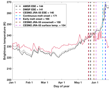
Figure 7. AMSR (black), DMSP (grey) and CESM2 JRA-55 (red) daily brightness temperatures in 2003 at approximately (a) 76 N, 168 W (b) 80 N, 140 E (c) 80 N, 80 E and (d) 84 N, 50 W. Dashed lines show the AMSR (black), DMSP (grey) and CESM2 JRA-55 (red) earliest snowmelt estimation dates (ESE) as well as the early melt onset date (light blue), the continuous melt onset date (dark blue), the CESM2 JRA-55 snowmelt melt onset date (brown) and the the CESM2 JRA-55 surface temperature melt onset date (pink).
