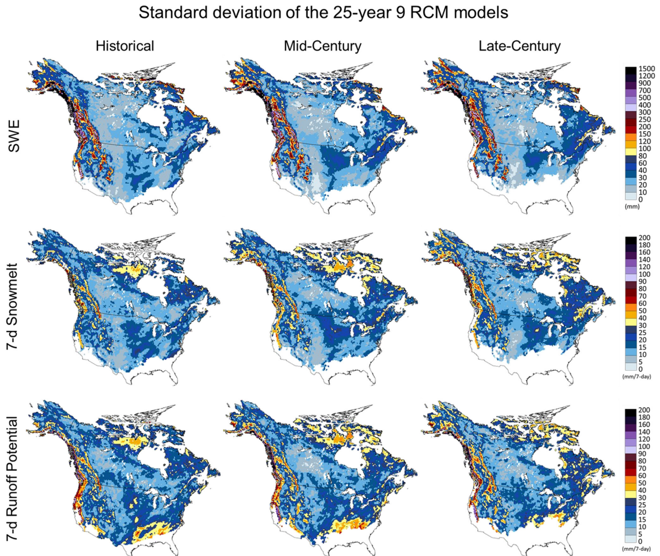
Figure 3. Standard deviations of the 25-year return level snow water equivalent (SWE), 7-day snowmelt, and runoff potential (RP) maps using the nine simulation outputs in the NA-CORDEX ensemble.
