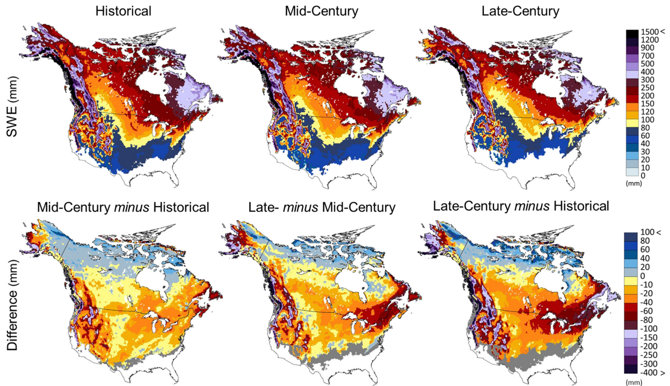
Figure 1. Twenty-five-year return level design snow water equivalent (SWE) using the annual maximum SWE values for the historical (1976–2005), mid (2040–2069), and late (2070–2099) century and their difference maps. Gray color along the southern edge in the difference maps indicates regions where the SWE no longer exists.
