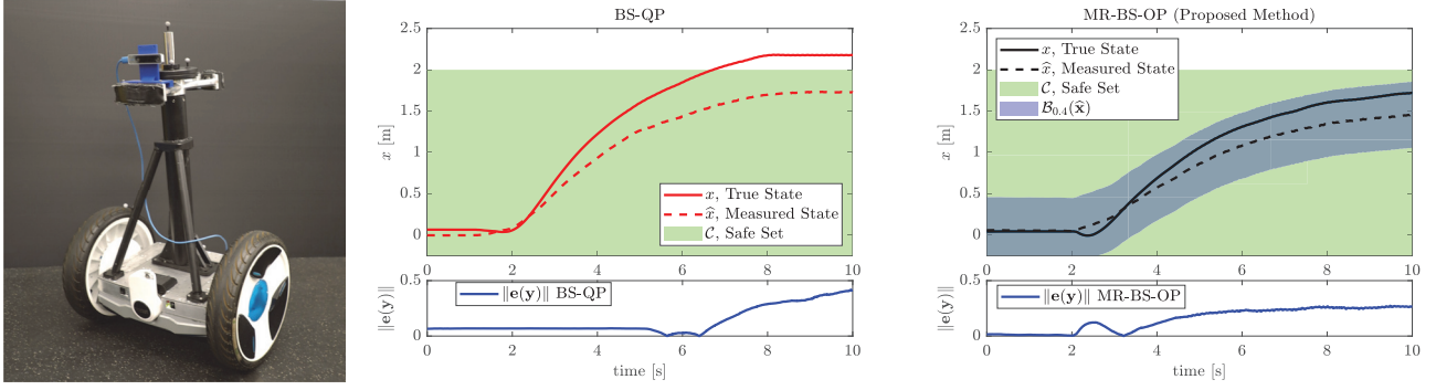
Fig. 3. Experimental results using SLAM from the onboard Intel RealSense T265 and constant desired velocity of 1 m/s. The notation and color schemes are the same as in Fig. 2. (Left) An image of the Segway platform. (Center) Trajectories generated using the BS-QP. The true trajectory exits the safe set at t = 6.7 s. The measurement error is plotted in blue. (Right) Trajectories generated using the MR-BS-OP. Both the true and measured trajectories are safe demonstrating the robustness of the MR-BS-OP when compared to the BS-QP.
