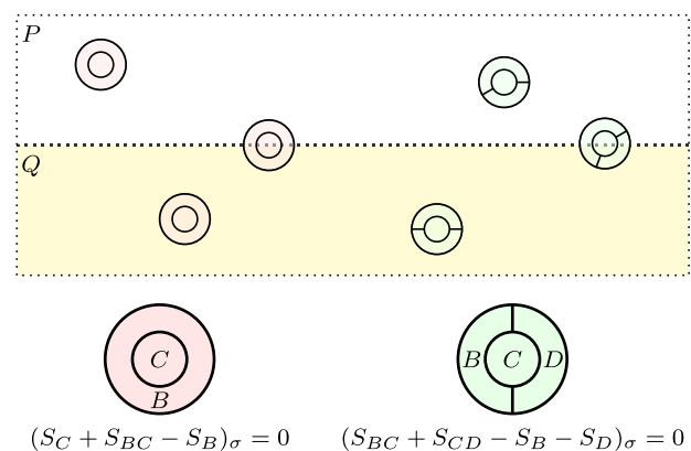
FIG. 1. Summary of our assumptions. We assume that (S_C + S_{BC} - S_B)_\sigma = 0 (red) and (S_{BC} + S_{CD} - S_B - S_D)_\sigma = 0 (green), both in the bulk and on the domain wall, over arbitrarily large regions that can be smoothly deformed from the shown configurations. Here, (\dots)_\sigma means that the entanglement entropies appearing in the parentheses is computed with respect to the reference state \sigma . The subsystems are allowed to be deformed as long as the boundaries between B and D do not cross the domain wall.
