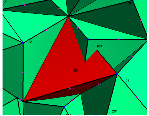
Figure 3: Example of edge-face intersection between element 152 (red) and element 103 (green).
