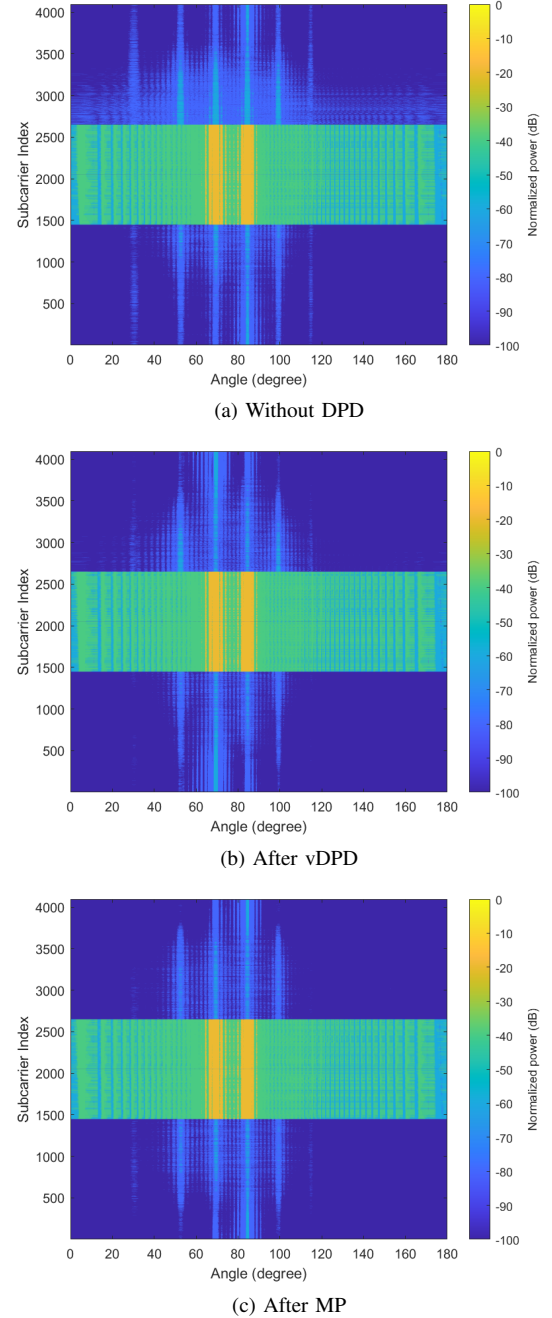
Figure 3. Radiated power as a function of angle and subcarrier for users placed at 70^\circ and 85^\circ from a ULA with N = 64 antennas. The subcarrier index corresponds to each 15 kHz bin used in the modulation. The center 1200 subcarriers correspond to in-band data. The lower subcarriers correspond to the first lower frequency OOB channel while the upper subcarriers correspond to the 1st upper frequency adjacent channel.
