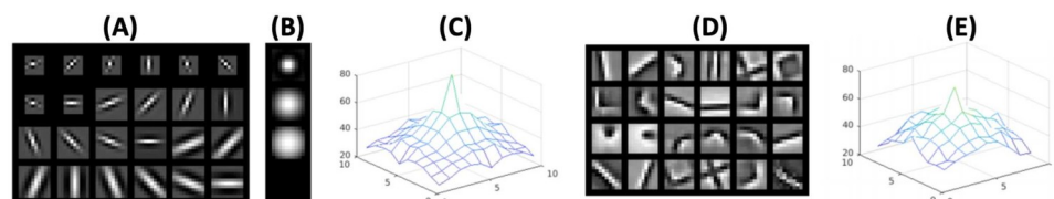
Fig 3. Gabor, Laplacian of Gaussian versus complex-shaped sparse code front-ends. From left to right we have: A: Gabor wavelets with 3 scales and 8 orientations. B: Laplacian of Gaussian kernels with 3 scales. C: The aggregated power spectrum of the Gabor wavelets. D: 24 complex-shaped sparse kernels selected from the 64-element CSC model for use in our Fixed Kernel CNN and Projection Pursuit models. E: Aggregated power spectrum of the complex-shaped sparse codes.
