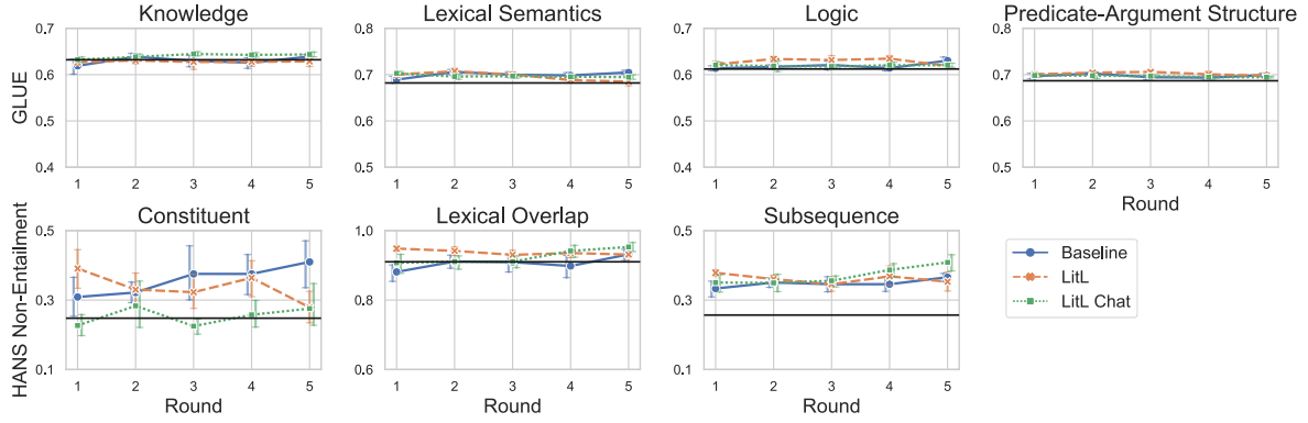
Figure 9: Performance of \text{RoBERTa}_{\text{Lg}+\text{MNLI}} fine-tuned on data collected through different protocols on the GLUE diagnostic set (top) and HANS non-entailment examples (bottom). The black line indicates performance of \text{RoBERTa}_{\text{Lg}} fine-tuned on MNLI alone. Error bars represent bootstrapped confidence intervals.
