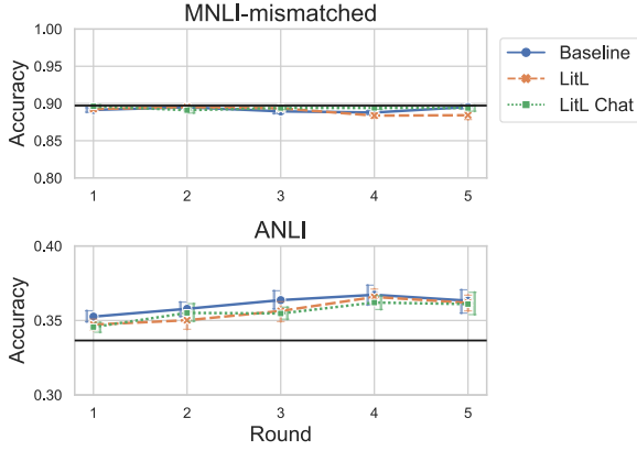
Figure 8: Performance of RoBERTa Lg +MNLI fine-tuned on data collected through different protocols on MNLI-mismatched (top) and ANLI (bottom). The black line for MNLI-mismatched and ANLI indicates performance of RoBERTa Lg fine-tuned on MNLI alone. Error bars represent bootstrapped confidence intervals.
