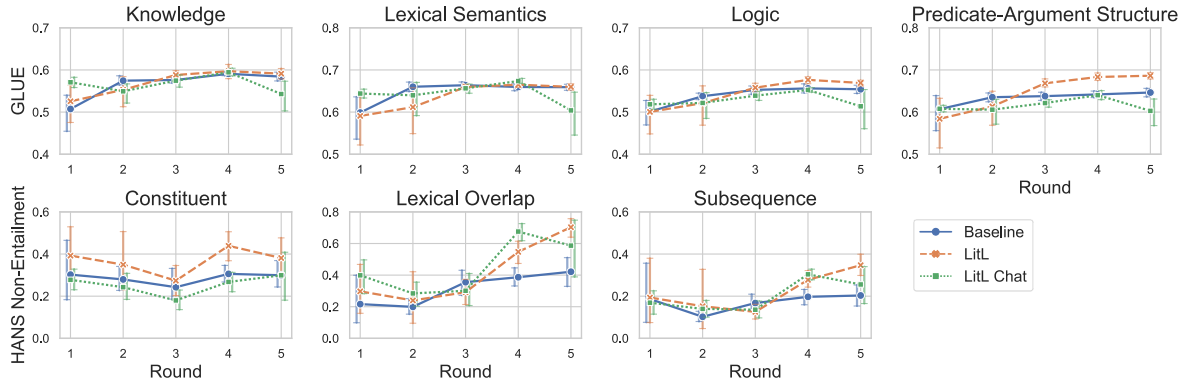
Figure 4: Performance of RoBERTa Lg fine-tuned on data collected through different protocols on the GLUE diagnostic set (top) and HANS non-entailment examples (bottom). Error bars represent bootstrapped confidence intervals.
