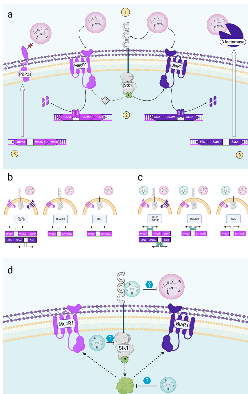
Figure 4. Brominated carbazoles disrupt \beta -lactam resistance gene transcription through an unknown mechanism. (a) MRSA utilizes combinations of PBP2a and \beta -lactamase to evade and inactivate \beta -lactam antibiotics. In step 1, \beta -lactam antibiotics (pink circle) bind to extracellular domains of MecR1, BlaR1, and Stk1. In step 2, the intracellular kinase domain of Stk1 phosphorylates the catalytic domain of BlaR1. BlaR1 cleaves BlaI and MecI , thereby permitting transcription of their respective operons. In step 3, transcription of blaZ and mecA leads to the formation of \beta -lactamase and PBP2a, respectively. (b) The four MRSA strains utilized in this work and their respective \beta -lactam resistance architectures are represented. 43300 and USA100 have full-length Stk1 , a functional bla operon, and Type II SCCmec, which confers a fully functional mec operon. USA300 does not have the bla operon and thus does not have BlaR1. USA300 possesses the Type IV SCCmec, causing a truncated MecR1 without the extracellular domain and no MecI . COL contains SCCmec I, which has the same MecR1 truncation as that in USA300. It does not contain the bla operon, and its stk1 has a premature stop codon that results in truncation of the extracellular domains. In each of these strains, treatment with \beta -lactam antibiotics (pink circle) leads to transcription of the mec operon and, if present, the bla operon. (c) Cotreatment with lead-brominated carbazoles (cyan circle) and \beta -lactam antibiotics (pink circle) dampens the transcription of bla and mec operons as compared with treatment with \beta -lactam alone in all MRSA strains with a full-length Stk1 . COL, which has a truncated Stk1 , shows no significant differential transcription of the mec operon upon cotreatment with \beta -lactams and lead brominated carbazoles. (d) On the basis of chemical genetics assays, we hypothesize that our lead carbazoles impact cellular signaling mechanisms that control the transcription of \beta -lactam resistance genes. Lead carbazoles may block antibiotic binding to the extracellular portion of Stk1, inhibit autophosphorylation or phosphotransfer from Stk1 to downstream targets, or inhibit signal transduction from a necessary second messenger protein that has yet to be elucidated.
