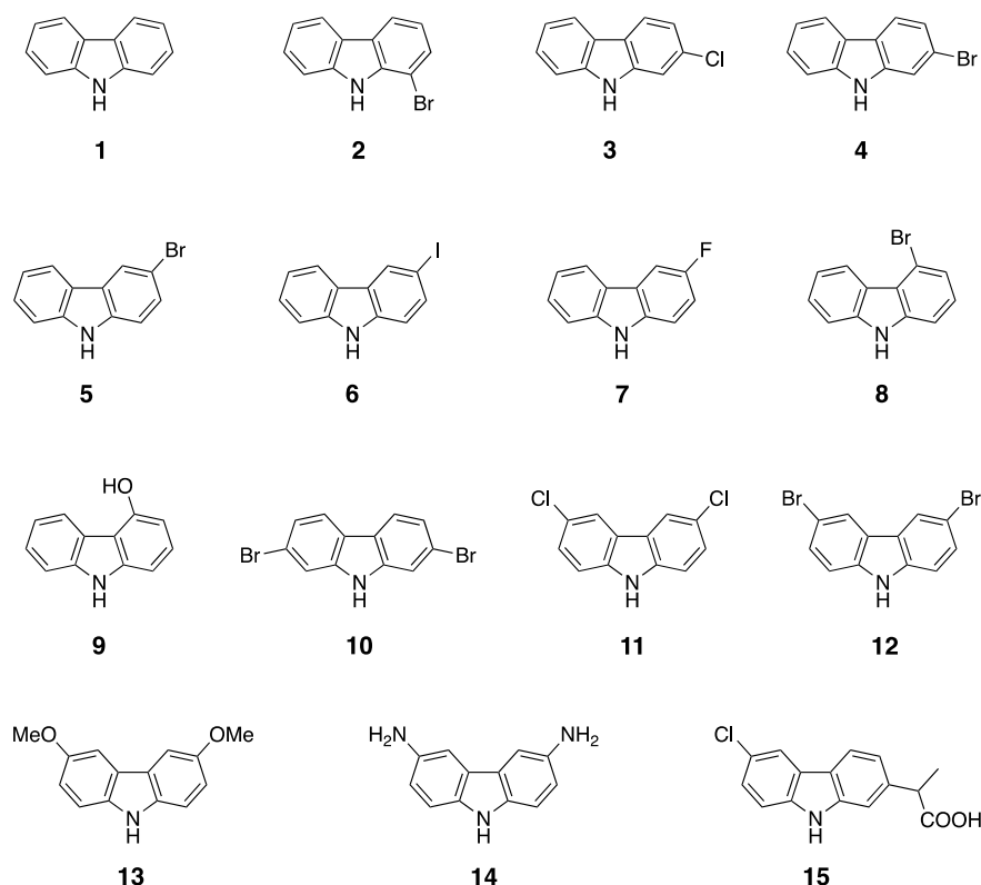
Figure 1. Library of commercially available carbazoles used to generate an initial structure–activity relationship (SAR).
