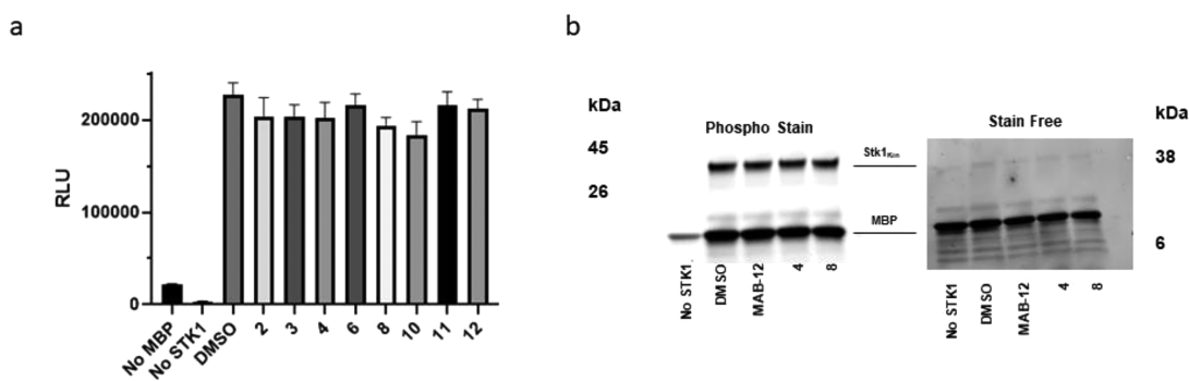
Figure 3. Carbazoles do not inhibit Stk1 kinase domain activity in vitro . (a) ADP-Glo assay of truncated Stk1 kinase domain and nonspecific phosphosubstrate myelin-basic protein (MBP) untreated (DMSO) or in the presence of 50 \mu\text{M} of the indicated compounds. RLU, relative luminescence units. Error bars represent the standard deviation of triplicate measurements. (b) Stk1 Kin was incubated with DMSO or 50 \mu\text{M} of the indicated compounds before the addition of ATP and MBP. No Stk1 Kin was used as a control.
