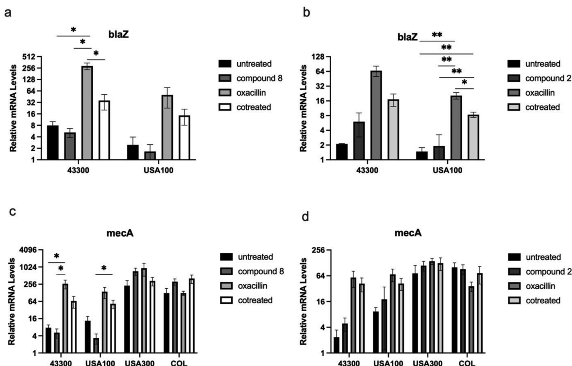
Figure 2. Cotreatment with carbazole compounds and oxacillin results in downregulation of blaZ and mecA . (a,b) Average levels of blaZ relative to 16S rRNA are displayed on a log2 scale. (c,d) Average levels of mecA relative to 16S rRNA are displayed on a log2 scale. In all panels, error bars represent the standard error of the mean. * p \leq 0.05 ; ** p \leq 0.01 . Compound 8 was assayed at 25 \mu\text{M} , and compound 2 was assayed at 50 \mu\text{M} .
