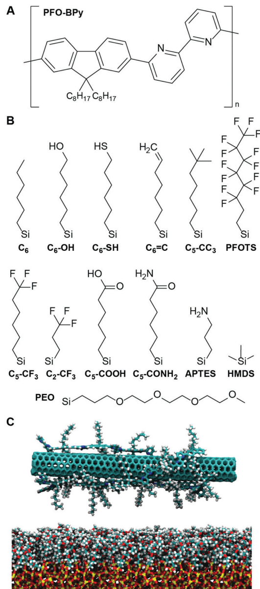
Fig. 1 A Chemical structure of PFO-BPy. B Chemical structures of ligands considered in this work, excluding alkylsilane ligands of which only -(CH_2)_5CH_3 , abbreviated as C 6 , is shown. The same nomenclature is used for other ligands. For example, C 6 -OH stands for -(CH_2)_6-OH . Ligands were grafted to form SAMs on silica substrates. C Snapshot from a MD simulation of a PFO-BPy-wrapped s-CNT near a PEO SAM in toluene. Silica is shown as yellow/red, PEO as cyan/red/white, PFO-BPy as cyan/blue/white, and the CNT in cyan. Toluene is not shown.
