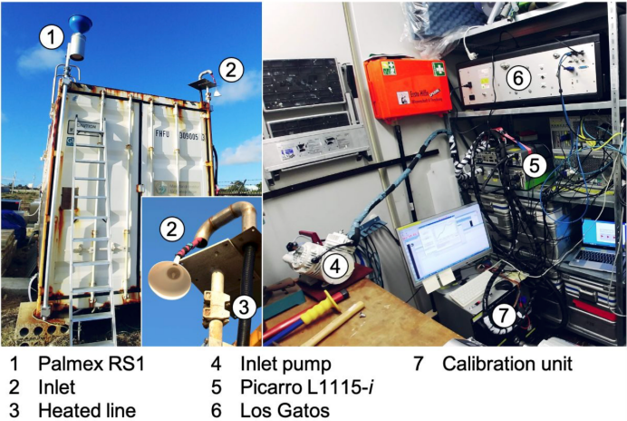
Figure 3: Isotopic sampling installations at the Barbados Cloud Observatory were comprised of a Palmex RS1 rainwater collector (#1) and two water vapor isotopic analyzers (fabricated by Picarro (#5) and Los Gatos Research (#6)).
