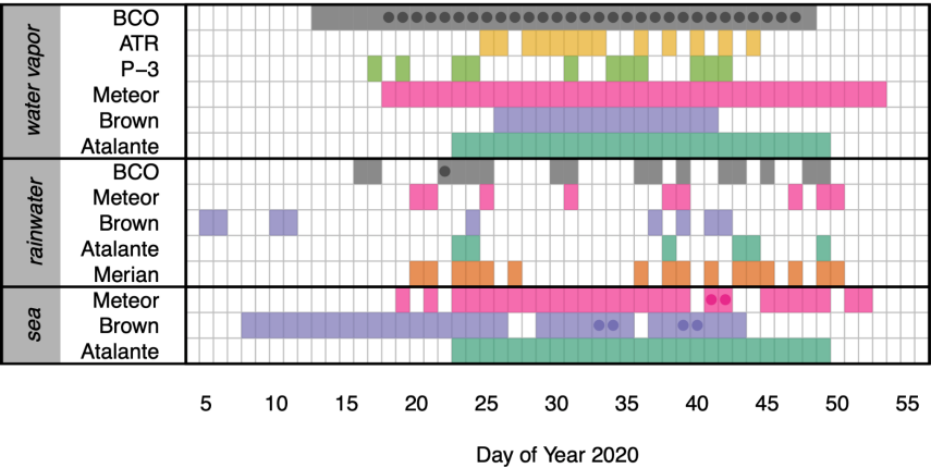
Figure 2: Timeline of continuous (water vapor) and discrete (rain and seawater) isotopic sampling during EUREC 4 A. Dots either represent days when two laser analyzers were operating at BCO or indicate intensive observation periods for rain or sea water (see main text for additional details). Discrete samples are represented by their collection times, which, in the case of Brown rainwater, were delayed in some cases by up to several days following precipitation.
