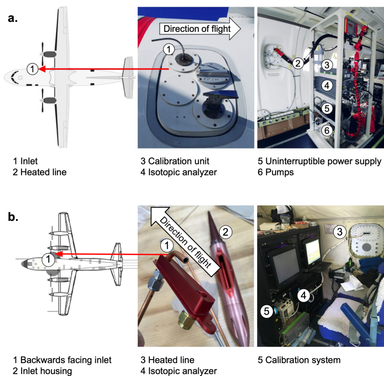
Figure 4: Water vapor isotopic sampling installations on the a) ATR and b) P-3 aircraft. (ATR schematic downloaded from https://t3projects.mpimet.mpg.de/coordination/platform-schematics . P3 schematic provided by NOAA.)
