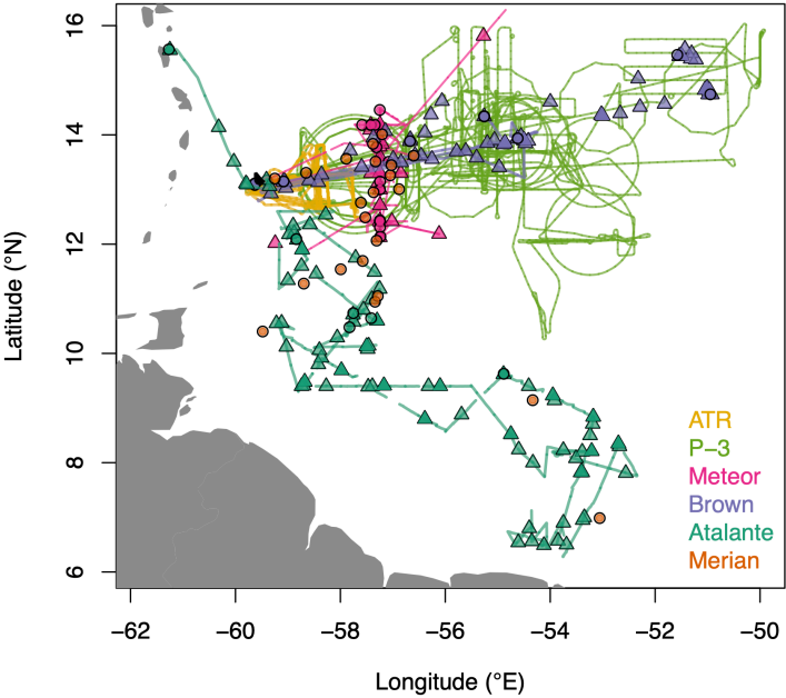
1255 Figure 1: Map of continuous (water vapor) and discrete (rain and seawater) isotopic sampling during the EUREC 4 A 2020 field experiment. Tracks for the various aircraft and ships are plotted only for periods during which water vapor isotopic sampling occurred. Circles and triangles indicate locations of rain and seawater sampling, respectively. Barbados appears in black.
