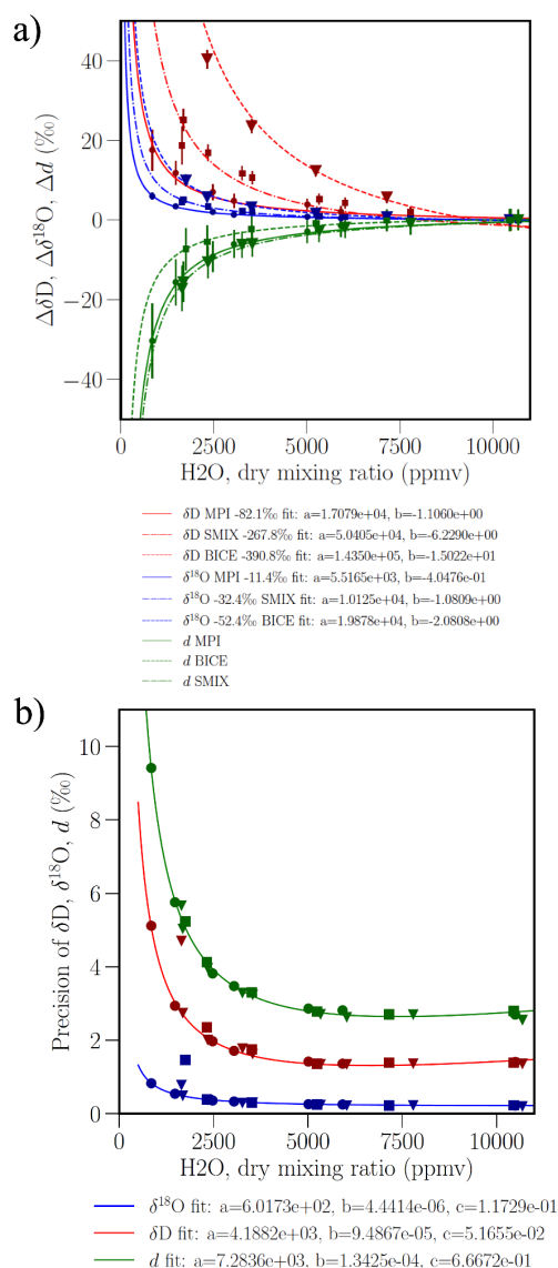
Figure 6: Bias corrections and uncertainties associated with the ATR water vapor isotopic measurements: a) symbols illustrate the humidity dependence of the isotopic measurements for three distinct liquid standards (MPI, SMIX, BICE) while lines show the correction functions used to remove the detected biases; b) precision of the isotopic measurements as a function of the measured water vapor concentration.
