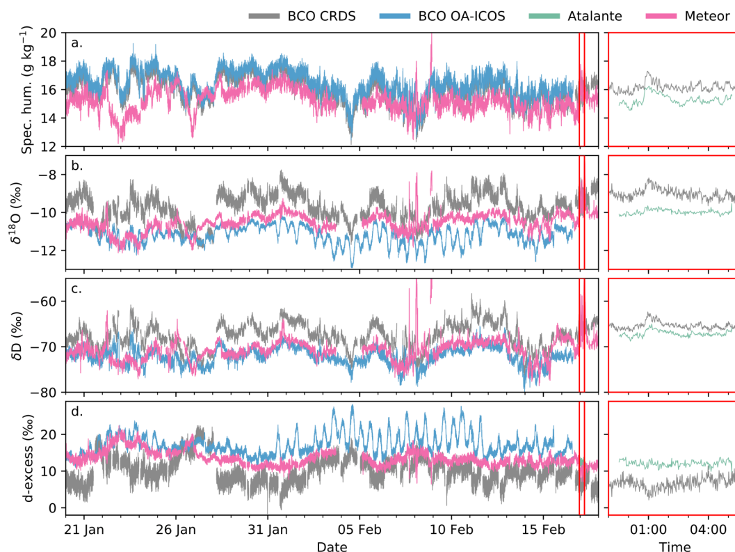
Figure 11: Time series of (a) water vapor concentration, (b) \delta^{18}\text{O} , (c) \delta\text{D} , and (d) d from the BCO CRDS analyzer (gray), the BCO OA-ICOS analyzer (blue), and the Meteor (magenta) for the period 20 January to 17 February 2020 (DOY 20-48). The Meteor trace is shifted by 9 hours. Rightmost panels show an enlarged view of the correlation between the BCO CRDS system and the Atalante (teal) for the period 23:30 16 Feb - 05:10 17 Feb UTC (DOY 47-48), when the Atalante was 1-3 nmi northeast of the BCO. The Atlante trace is shifted by 10 minutes.
