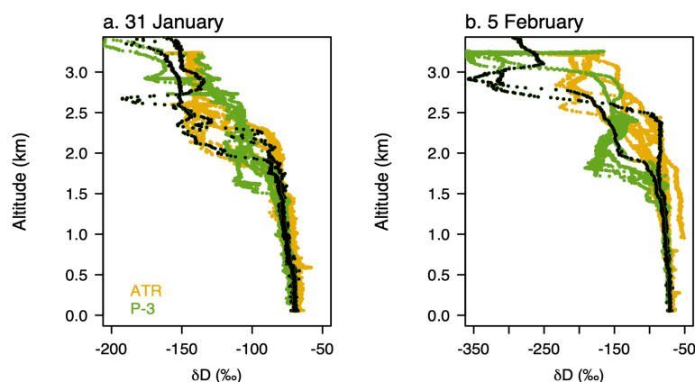
1325 Figure 12: Vertical \delta D profiles from the ATR (yellow) and the P-3 (green) for (a) 31 January (DOY 31) and (b) 5 February (DOY 6), the two days on which both aircraft were in the air simultaneously. P-3 observations with black centers represent takeoffs and landings, which were flown in closest proximity to the ATR and show the greatest structural similarity to ATR \delta D profiles.
