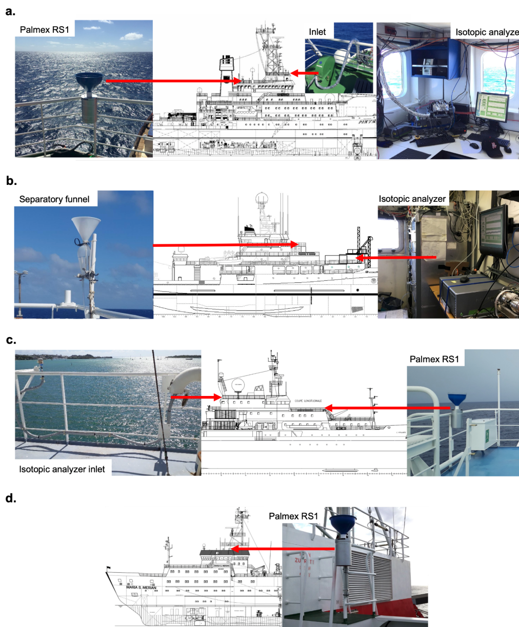
Figure 5: Water isotopic sampling installations aboard a) the Meteor, b) the Brown, c) the Atalante, and d) the Merian. (Meteor and Merian ship schematics provided by University of Hamburg. Brown ship schematic provided by NOAA. Atalante ship schematic copyright ©Ifremer. Atalante photos courtesy of Jérôme Demange.)
