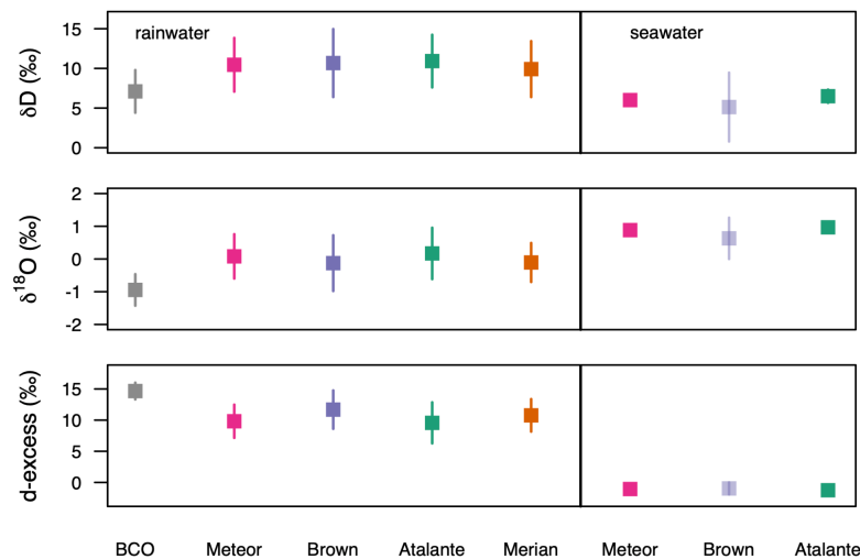
Figure 10: Campaign-mean rainwater and seawater values from the BCO and ship-based platforms. Whiskers represent standard deviations. Flagged samples and seawater samples taken from a depth greater than 10 m are excluded from the comparison. Brown seawater values are still preliminary and laboratory analysis of Brown seawater ongoing.
