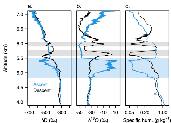
Figure 8: Strong hysteresis causes (a) the \delta D vertical profile to differ substantially from vertical profiles of (b) \delta^{18}O and (c) specific humidity during P-3 Research Flight 8. Three dry layers, in which the delayed response and weaker signal in \delta D are most evident, are indicated by shading. Signal delay is most evident on the descending profile (black). \delta^{18}O is characterized by a better time response than \delta D but shows unphysical enrichment at altitude due to a shifting humidity-dependent bias over the course of the campaign.
