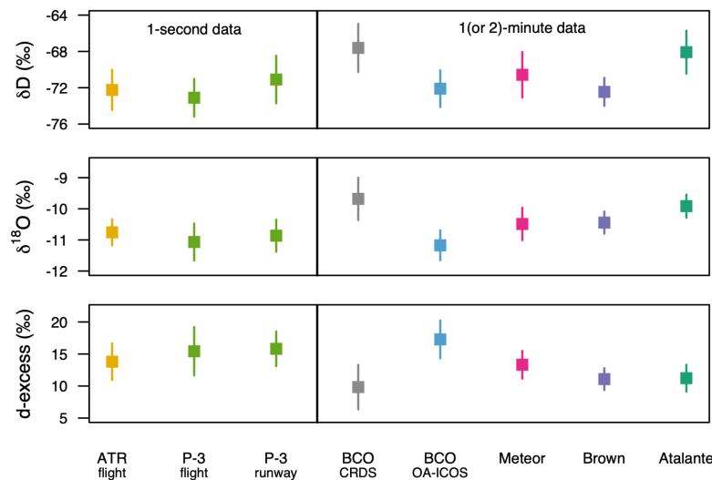
Figure 9: Campaign-mean near-surface water vapor isotopic values from the various ground, airborne, and ship-based platforms. Whiskers represent standard deviations. Values from in flight represent a height of 150±15 m.a.s.l. Only non-flagged data included in the comparison.
