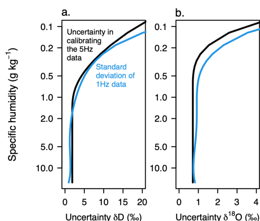
Figure 7: P-3 isotopic uncertainties (x-axis) plotted as a function of specific humidity (y-axis). The y-axis is plotted on a logarithmic scale to convey the approximate uncertainties of the vertical profiles measured by the aircraft. Black lines indicate uncertainties associated with the normalization of the 5 Hz data to the VSMOW-SLAP scale. Blue lines represent the standard deviations associated with the 1 Hz averages from the first two research flights: they reflect both the variability of the environment and the additional imprecision of the isotopic analyzer in flight.
