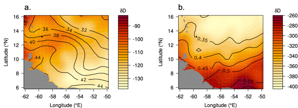
1330 Figure 13: a) TROPOMI total column \delta D (shading) and total column water ( \text{kg m}^2 , contours), averaged on a 0.5-degree grid and smoothed for the period 11 Jan - 20 Feb 2020 (DOY 11-51). Only retrievals with a quality value of 0.5 or higher are selected. b) IASI \delta D and specific humidity ( \text{g kg}^{-1} ; contours) at 6.4 km, averaged on a 0.5-degree grid and smoothed for the same period. (Note that the two water vapor fields represent distinct quantities.) Only data marked “good quality” 1335 in terms of spectral fit are used. Barbados appears in black.
