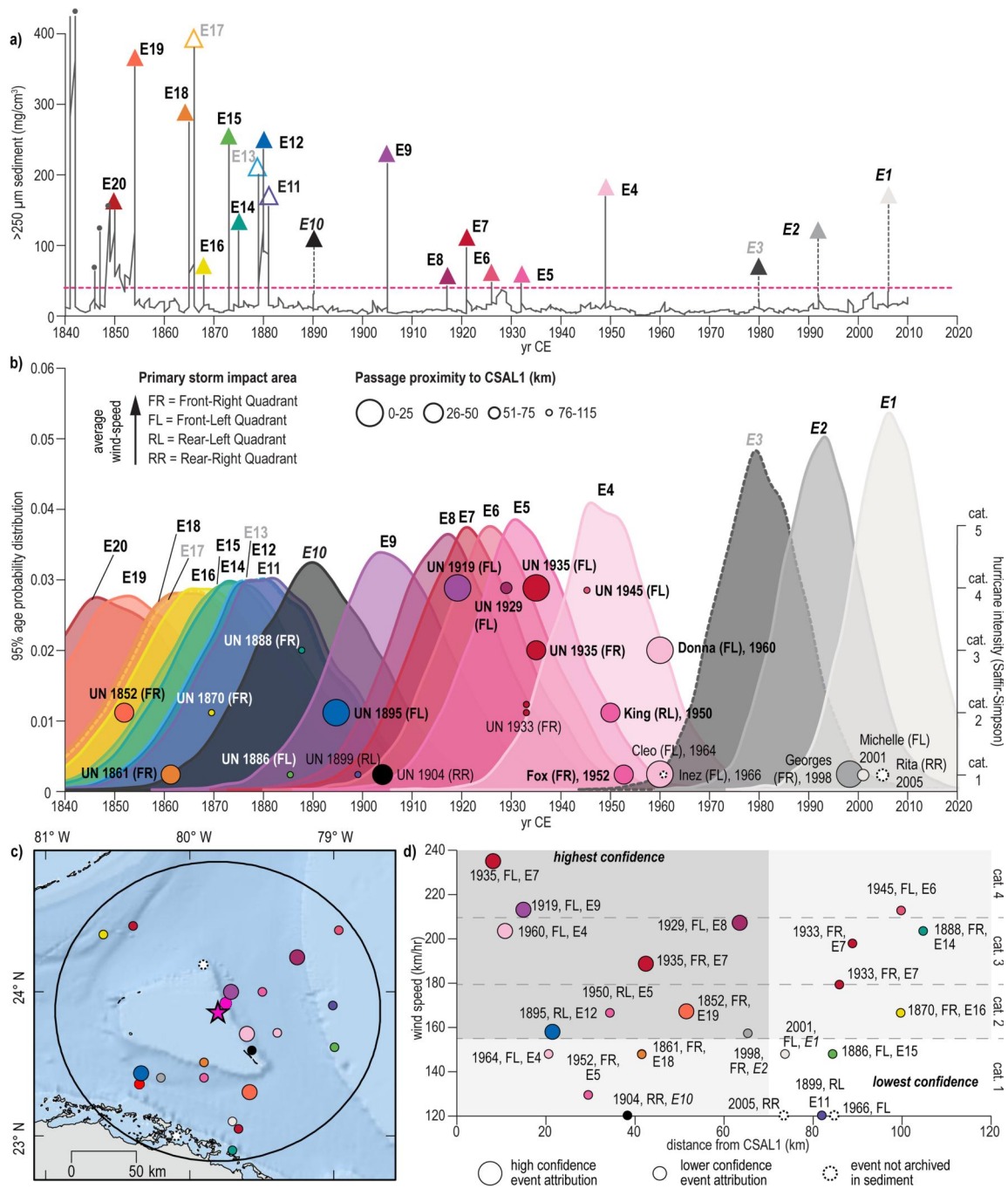
Fig. 6. a) Coarse sediment data ( \text{mg}/\text{cm}^3 ) > 250 \mu\text{m} , in dark grey and > 63 \mu\text{m} in light grey) with > 40.9 \text{ mg}/\text{cm}^3 > 250 \mu\text{m} coarse anomaly event beds E-1, E2, E3, and E10 (from Cores-8 and 9) and E4-E19 indicated respectively by greyscale and colored triangles that correspond to the colors of 95% age probability distribution (95% PDF) plots in panel b). Only the > 250 \mu\text{m} data was used to define hurricane event beds, but the most prominent peaks are also observed in the > 63 \mu\text{m} data. Circles on panel b) correspond to the timing of hurricanes observed within 115 km of Hine's Hole from 1850 to 2015 CE ( n = 23 ). Circle diameter is proportional to passage proximity (larger circle = closer passage), and vertical position of the circles corresponds to the intensity of the storm on the Saffir-Simpson hurricane scale (right y-axis). Circle colour corresponds to the colour of the 95% PDF plot of the event bed that the observed hurricane event is most likely associated with (modern hurricanes with no associated event bed in the Hine's Hole Composite are solid black). Panel c) includes a map of the point of closest passage to Hine's Hole of all hurricanes from 1850 to 2015 CE depicted in panel b), with colour associated with the coarse anomaly that is attributed to the hurricane event and the size and shape corresponding to the confidence in that attribution (see legend). Applying the same symbology, d) is a scatterplot of the wind speed of each of these hurricanes plotted against to the distance of closest passage to Hine's Hole. This diagram shows that over the last \sim 170 years, Hine's Hole reliably archives most \geq Category 1 hurricanes within 75 km and most \geq Category 2 hurricanes within 115 km depending on the angle of approach.
