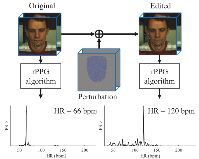
Fig. 1. PulseEdit can edit the rPPG signal in a facial video to conceal a person’s true physiological status, without visual distortion of his/her appearance. We introduce negligible additive perturbations onto the facial region in the video, and successfully modify the HR extracted by the rPPG algorithm. In this example, HR is edited from 66 to 120 beats per minute (bpm) to avoid the disclosure of the user’s true heart rate in the video.
