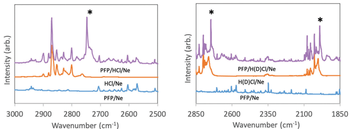
Fig. 1 IR spectra of neon matrices containing pentafluoropyridine (PFP) and/or H(D)Cl. Left: HCl/PFP/Ne at guest–host ratios of 1/1/1600; controls at 1/800. Right: H(D)Cl/PFP/Ne at guest host ratios of 2*/1/1600 (*with an approximate 1/1 relative concentration D/H); controls at 1/800 (PFP) and 1/400 H(D)Cl.
