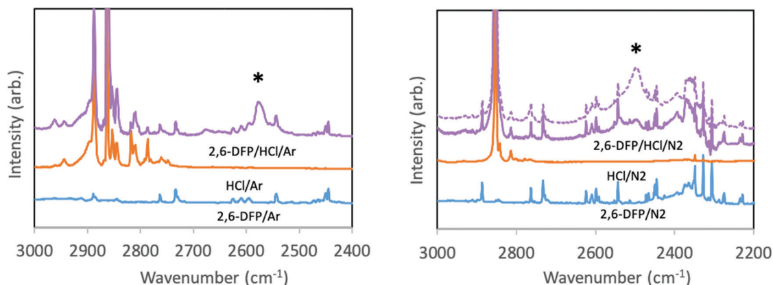
Fig. 4 IR spectra of argon and matrices containing 2,6-difluoropyridine (2,6-DFP) and HCl. Left: HCl/2,6-DFP/Ar at guest–host ratios of 1/1600; controls at 1/800. Right: HCl/PFP/N 2 at guest host ratios of 1/800 for the control spectra, and 2/3/4000 for the sample with both HCl and 2,6-DFP. Dashed line is annealed sample (30 min at 28 K).
