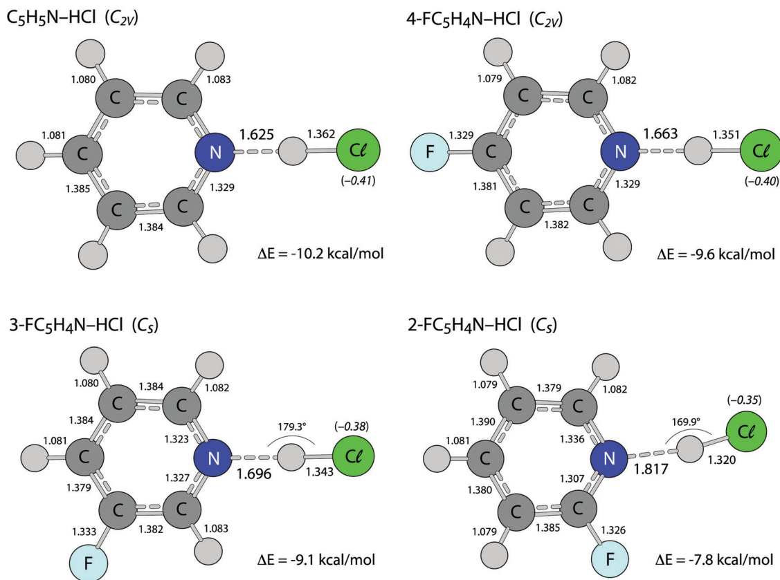
Fig. 7 Equilibrium structures and binding energies for C_5H_5N-HCl and its singly fluorinated analogs at the \omega B97X-D/aug-cc-pVTZ level of theory. Interatomic distances are displayed in units of Å. Charges on the chlorine atoms were obtained from Natural Population Analyses, and are included in parentheses (in units of e).
