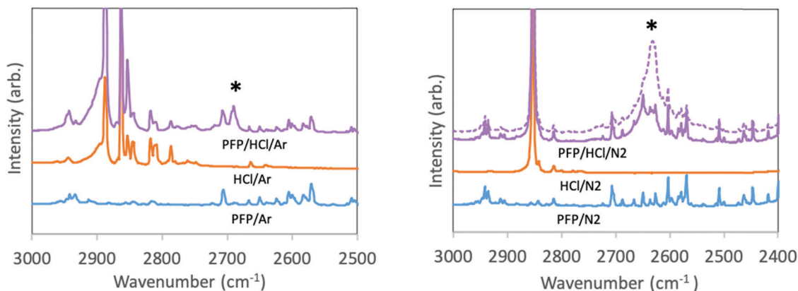
Fig. 2 IR spectra of argon and matrices containing pentafluoropyridine (PFP) and HCl. Left: HCl/PFP/Ar at guest–host ratios of 1/1/1600; controls at 1/800. Right: HCl/PFP/N 2 at guest host ratios of 1/800 for the control spectra, and 3/4/5600 for the sample with both HCl and PFP. Dashed line is annealed sample (30 min at 28 K).
