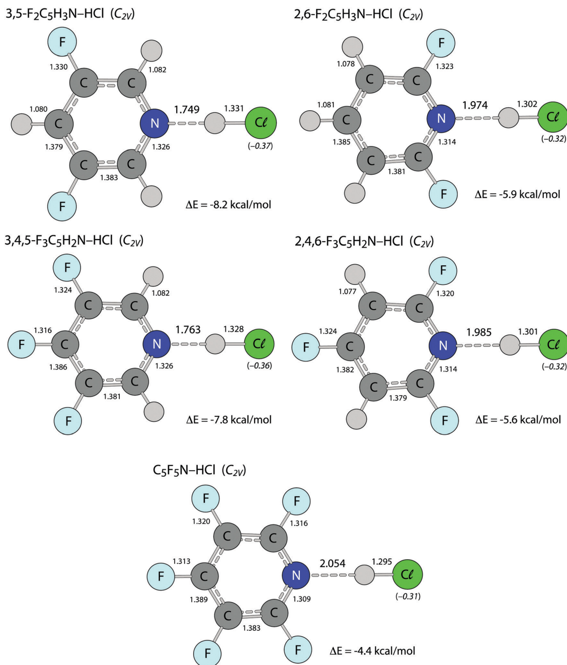
Fig. 8 Equilibrium structures and binding energies for the difluoro-, trifluoro-, and pentafluoro-pyridine-HCl complexes, at the \omega B97X-D/aug-cc-pVTZ level of theory. Interatomic distances are displayed in units of Å. Charges on the chlorine atoms were obtained from Natural Population Analyses, and are included in parentheses (in units of e ).
