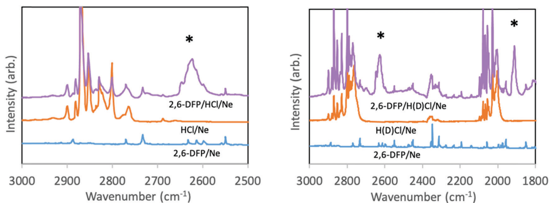
Fig. 3 IR spectra of neon matrices containing 2,6-difluoropyridine (2,6-DFP) and/or H(D)Cl. Left: HCl/2,6-DFP/Ne at guest–host ratios of 1/1/1600; controls at 1/800. Right: H(D)Cl/2,6-DFP/Ne at guest host ratios 3*/2/4000 for the sample with both HCl and PFP; 2*/800 and 1/800 for the controls, respectively (* with an approximate 1/1 relative concentration D/H).
