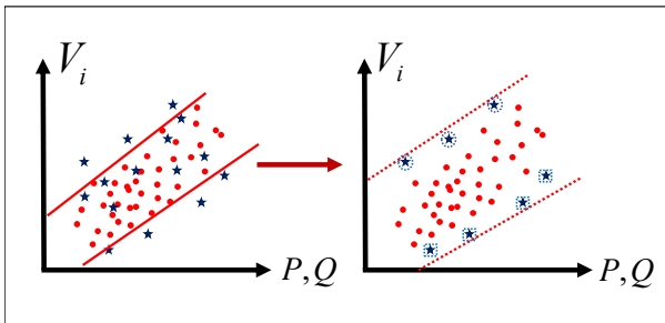
Fig. 1. An example of the sample selection method. The red circles and the blue stars are the previous and the new samples, respectively. The top (bottom) lines illustrate over- (under-) estimating CLAs. The right picture shows that only new samples which violate the previous CLA are included to compute the updated CLA. Specifically, the stars with the dashed circles (squares) are included for the updated over- (under-) estimating CLA.
