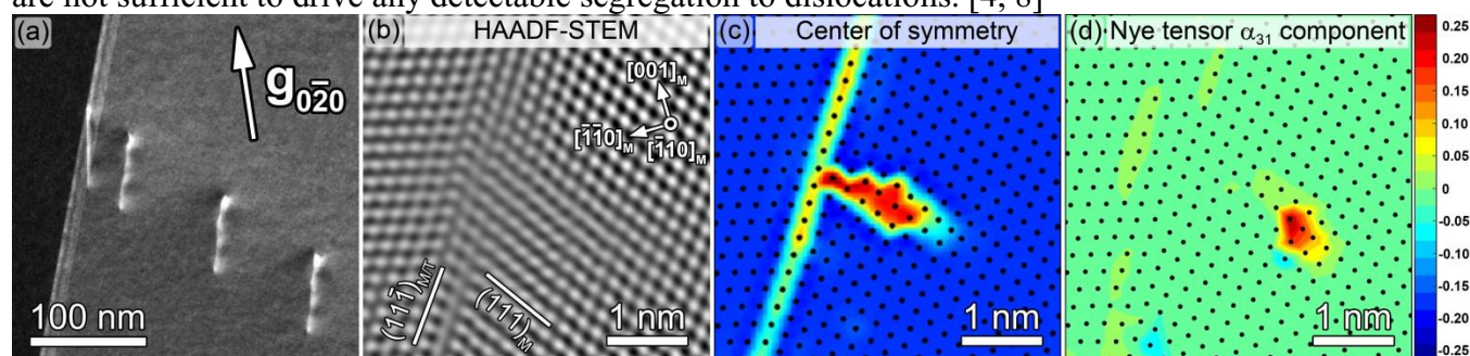
Figure 1. Figure 1. (a) Planar dislocation slip with the screw dislocation at the head of the pile-up oriented parallel to the crystallographic direction. (b) HAADF-STEM showing the core of a 1/2 dislocation in the equiatomic CrMnFeCoNi alloy after tensile pre-deformation and annealing at 973K for 800 hours. Corresponding (c) COS and (d) \alpha_{31} Nye tensor map.[4]
