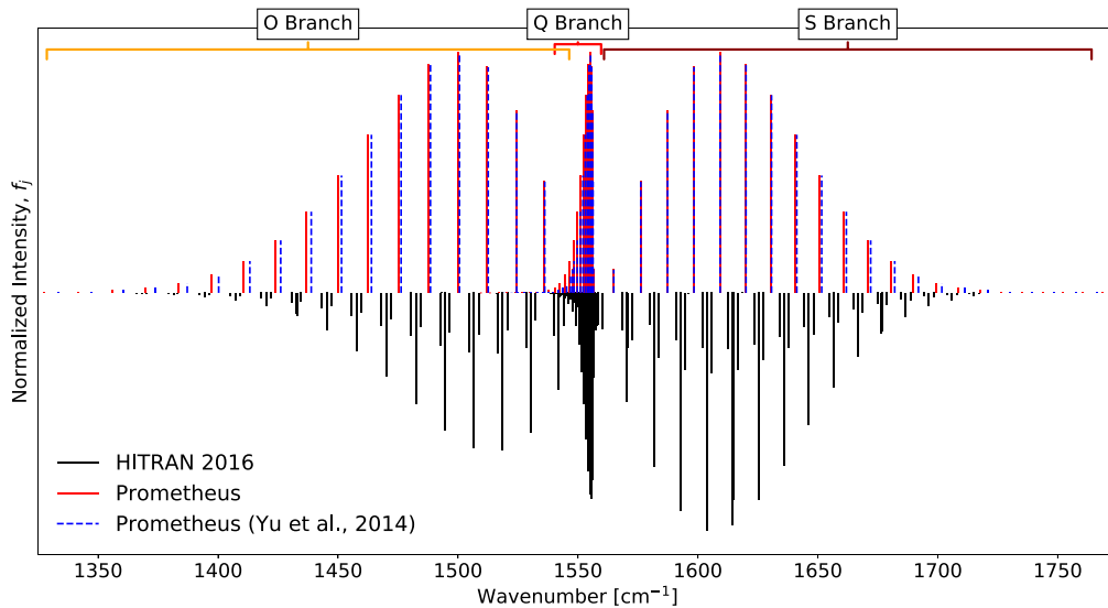
Figure 4. A comparison of the O_2 spectra produced by Prometheus, Prometheus using the spectroscopic constants from Yu et al. (2014) and HITRAN 2016 data (Gordon et al. 2017; Gamache et al. 1998; Yu et al. 2014). The intensities for all sets of data have been normalized and therefore are relative values.
