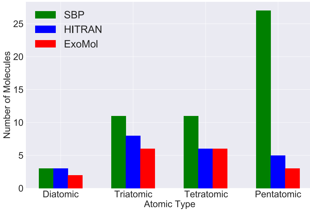
Figure 1. Comparing the availability of data from HITRAN and ExoMol with the molecules needed for the SBP. Only up to pentatomic molecules have been included here.
