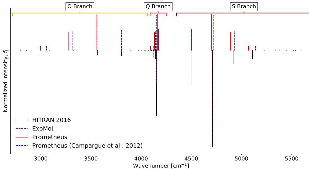
Figure 2. A comparison of the H_2 spectra produced by Prometheus, ExoMol (Roueff et al. 2019), and Prometheus using the spectroscopic constants from Campargue et al. (2012). The intensities for all sets of data have been normalized and therefore are relative values. Note that HITRAN and ExoMol transitions overlap with each other.
