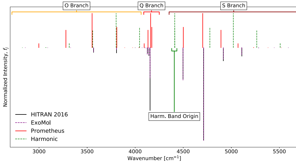
Figure 3. A comparison of the \text{H}_2 spectra produced by Prometheus, ExoMol (Roueff et al. 2019) and the Harmonic method. The intensities for all sets of data have been normalized and therefore are relative values. Note that HITRAN and ExoMol transitions overlap with each other.
