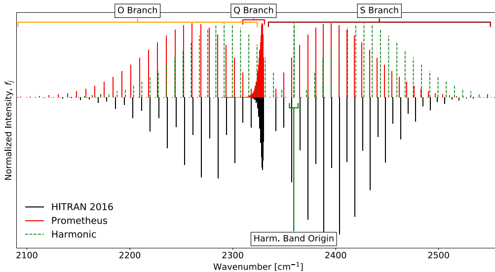
Figure 7. A comparison of the N_2 spectra produced by Prometheus, the harmonic method, and HITRAN 2016 (Roy et al. 2006; Li & Roy 2007; Gordon et al. 2017) data. The intensities for all sets of data have been normalized and therefore are relative values.
