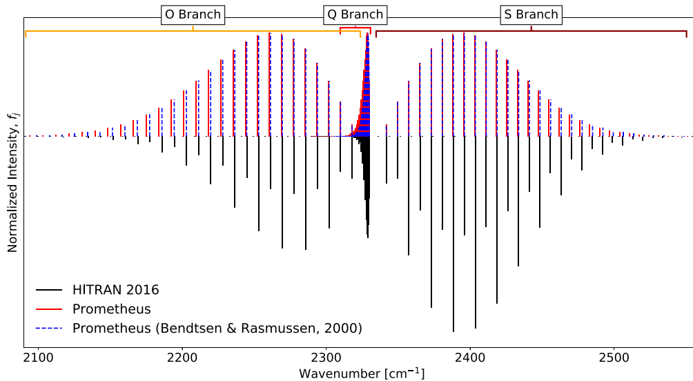
Figure 6. A comparison of the N_2 spectra produced by Prometheus, Prometheus using the spectroscopic constants from Bendtsen & Rasmussen (2000), and HITRAN 2016 (Gordon et al. 2017; Li & Roy 2007; Roy et al. 2006) data. The intensities for all sets of data have been normalized and therefore are relative values.
