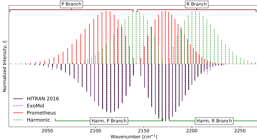
Figure 9. A comparison of the CO spectra produced by Prometheus, the harmonic method, ExoMol (Li et al. 2015), and HITRAN 2016 data (Coxon & Hajigeorgiou 2004; Li et al. 2015; Gordon et al. 2017; Devi et al. 2018). The intensities for all sets of data have been normalized and therefore are relative values.
