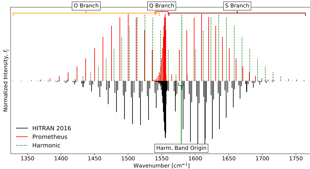
Figure 5. A comparison of the O_2 spectra produced by Prometheus, the harmonic method, and HITRAN 2016 data (Gamache et al. 1998; Yu et al. 2014; Gordon et al. 2017). The intensities for all sets of data have been normalized and therefore are relative values.
