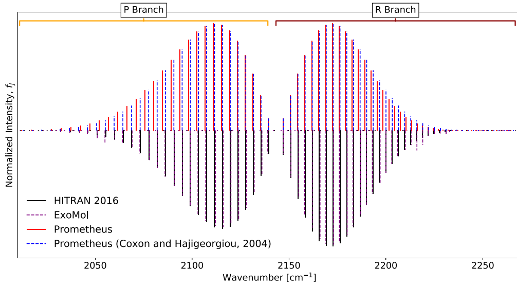
Figure 8. A comparison of the CO spectra produced by Prometheus, Prometheus using the spectroscopic constants from Coxon & Hajigeorgiou (2004), ExoMol (Li et al. 2015), and HITRAN 2016 data (Coxon & Hajigeorgiou 2004; Li et al. 2015; Gordon et al. 2017; Devi et al. 2018). The intensities for all sets of data have been normalized and therefore are relative values.
